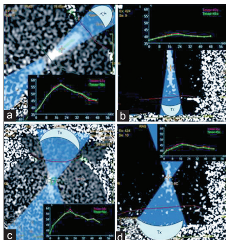
Figure 5: Thermal spot shapes as seen on Cadaver 2 and tissue mimicking phantom. a,c-sonication on Thiel embalmed cadaver with and ó of the transmitting transducer, respectively. b, d- sonication on phantom with the same parameters as been used for cadaver sonications
