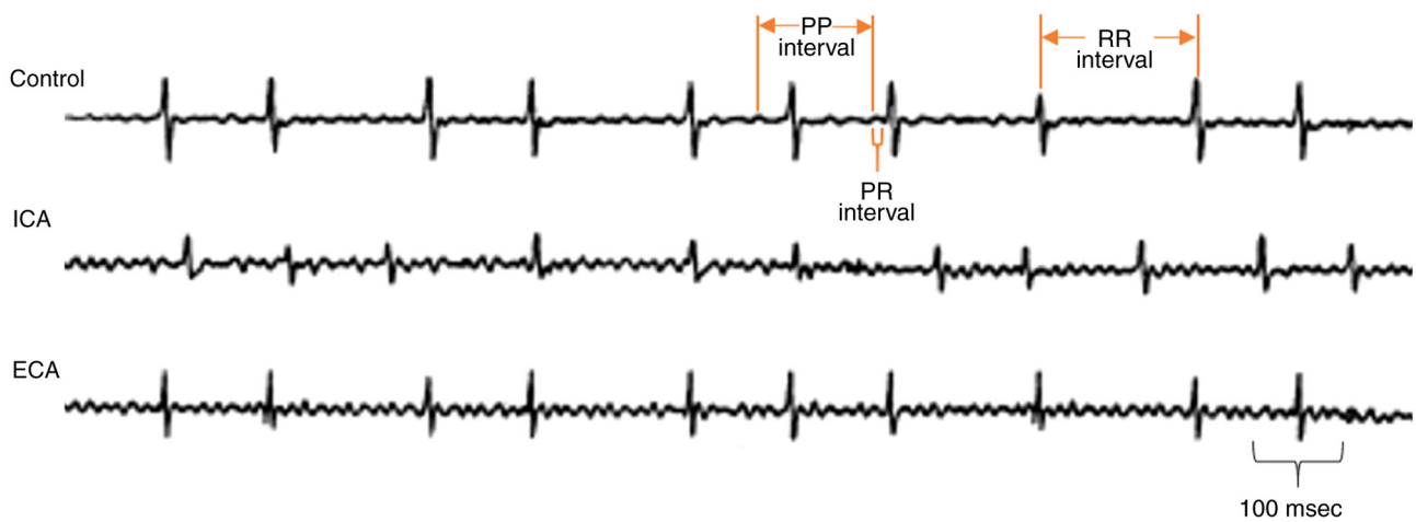
Figure 1. ECGs of leptin receptor-deficient mice at the initial and end stages of cardiac arrhythmia. The ECGs show progressive variation of the PP interval with increasing severity of cardiac arrhythmia, and variations in each beat, as evidenced by variable PP and PR intervals. ECGs, electrocardiograms; ICA, initial-stage cardiac arrhythmia; ECA, end-stage cardiac arrhythmia; PP interval, average time between successive P waves; PR interval, average time from the onset of the P wave to the start of the QRS complex; RR interval, average time between QRS complexes.
