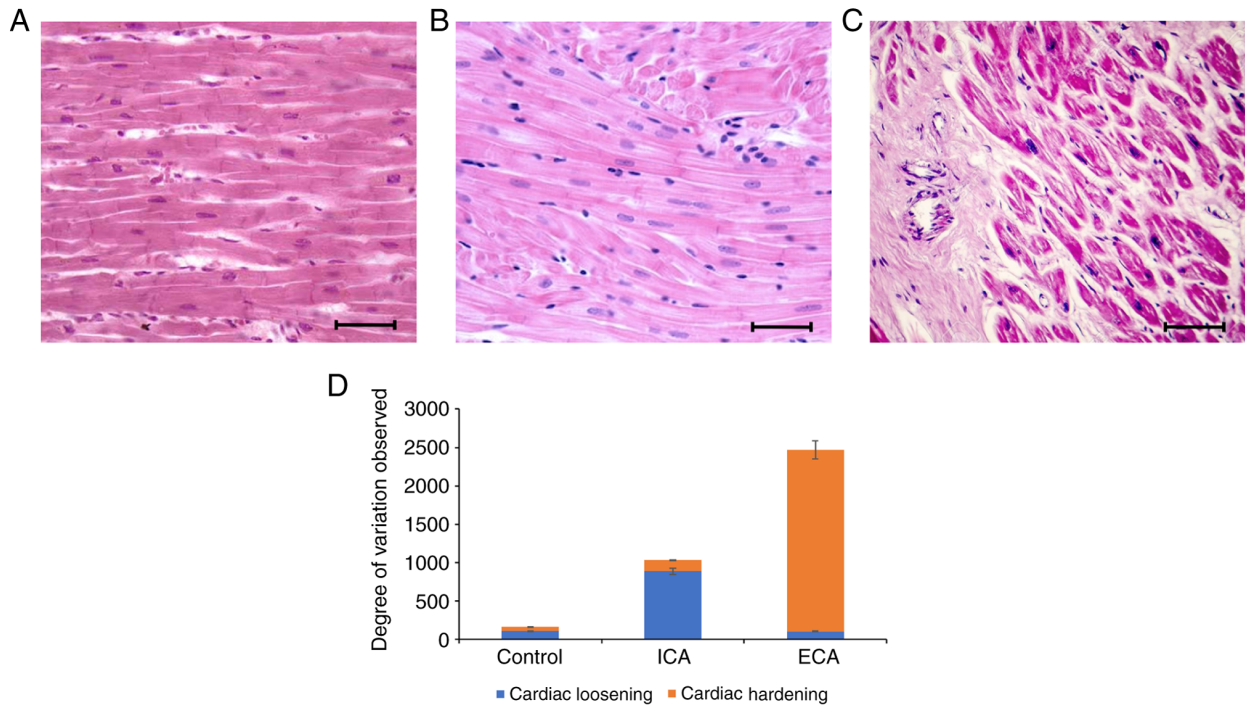
Figure 2. Histological variations in the cardiac tissue from mice at various stages of cardiac arrhythmia. (A) Normal mouse cardiac tissue, showing a compact cellular structure, with prominent nuclei. (B) Cardiac tissue from a mouse with ICA, showing a loosened cellular structure with a scattered appearance. (C) Cardiac tissue from a mouse with ECA, showing a complete change in cellular morphology, together with tissue hardening. Hematoxylin and eosin staining. Scale bar, 100 \mu m. (D) Graphical representation of histological variations observed in mouse cardiac tissue at the initial and end stages of cardiac arrhythmia compared with those of normal mice. ICA, initial-stage cardiac arrhythmia; ECA, end-stage cardiac arrhythmia.
