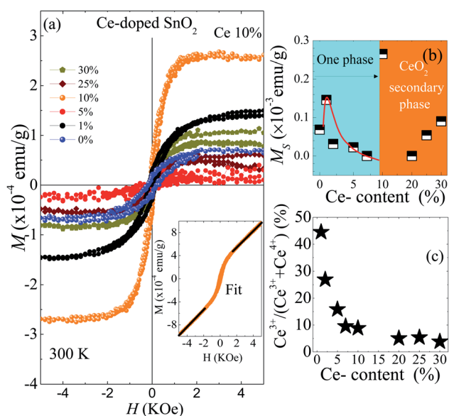
Fig. 4 (a) Magnetization curves for the undoped and Ce-doped SnO 2 NPs (the inset shows the magnetization signal before subtracting the paramagnetic and diamagnetic contributions in the 10% Ce-doped NPs). (b) Saturation magnetization of the ferromagnetic contribution as a function of the Ce content. (c) Percent of Ce 3+ -ions as a function of the Ce content.
