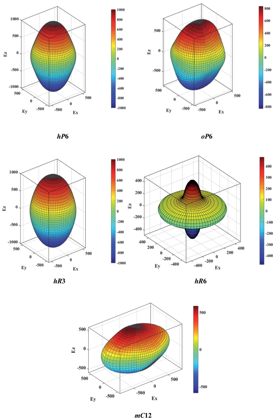
Fig. 4 The direction-dependent Young's modulus of \text{ReB}_2 in different crystal structures.
