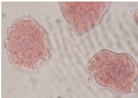
FIGURE 3: Ghost cells.
