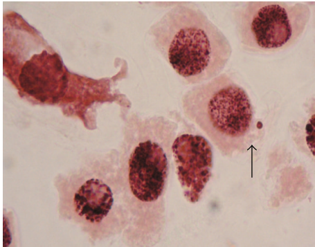
FIGURE 2: Micronucleus.
