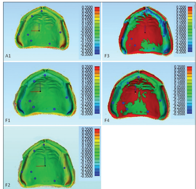
Figure 3: Color maps of intaglio surface of maxillary denture base. Nominal deviation (green); positive deviation (yellow to red) misfit with space; negative deviation (cyan to blue) tissue compression
