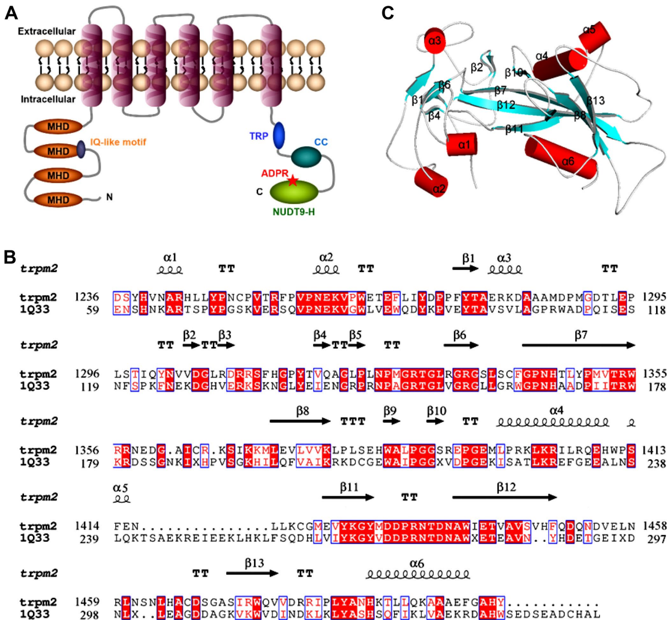
Figure 1. Homology modeling of the NUDT9-H domain from the human TRPM2 channel protein. (A) Schematic diagram showing the membrane topology of the TRPM2 channel proteins. Important domains are labeled in the figure. (B) Sequence alignments of the human NUDT9 and NUDT9-H domain. Red shading with purple border denotes identical residues, and white shading with purple border denotes similarities. (C) Ribbon presentation of the homology models of the NUDT9-H domain based on the human NUDT9 structure. The \alpha -helices, \beta -sheets, and loops are labeled in red, cyan, and gray, respectively.
