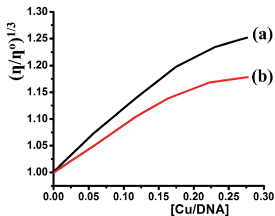
Fig. 16 Effect of concentration of (a) complex 1 and (b) complex 2 [ 0, 2.5 \times 10^{-5}, 6.25 \times 10^{-5}, 8.75 \times 10^{-4}, 1.12 \times 10^{-4}, and 1.37 \times 10^{-4} M] on relative viscosity of CT-DNA ( 5 \times 10^{-4} M) at RT in Tris-HCl buffer.
