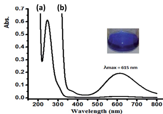
Fig. 9 UV-Vis spectra recorded for complex 1 dissolved in water at RT at a concentration of (a) 5 \times 10^{-5} M and (b) 5 \times 10^{-4} M.
