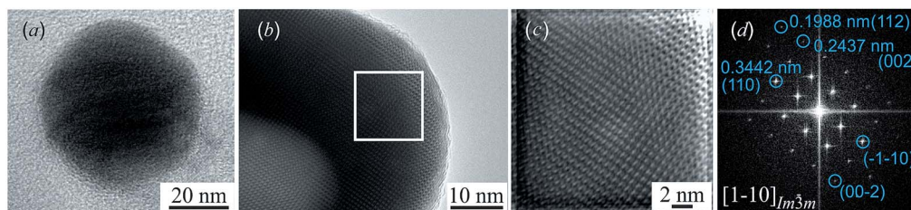
Fig. 6 (a) TEM image of a separate \text{Ag}_2\text{S} nanoparticle; (b) HRTEM image of the \text{Ag}_2\text{S} nanoparticle with a cubic (space group Im\bar{3}m ) \beta - \text{Ag}_2\text{S} argentine structure; (c) a part of the HRTEM image, isolated by a white rectangle, at larger magnification; (d) electron diffraction pattern (zone axis [1-10]Im\bar{3}m ) obtained by FFT of the HRTEM image area in the white rectangle.
