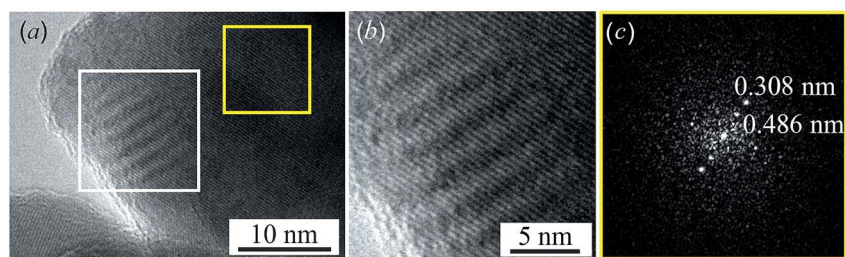
Fig. 4 HRTEM image (a) of an \text{Ag}_2\text{S} nanoparticle heated by an electron beam to a temperature T of about 450–451 K; Moiré fringes are clearly visible near the edge of the nanoparticle. (b) Magnified HRTEM image of the nanoparticle area, highlighted by a white square in (a), with wave-like Moiré fringes. (c) Electron diffraction pattern obtained by FFT of the HRTEM image of the nanoparticle area highlighted by a yellow square in (a).
