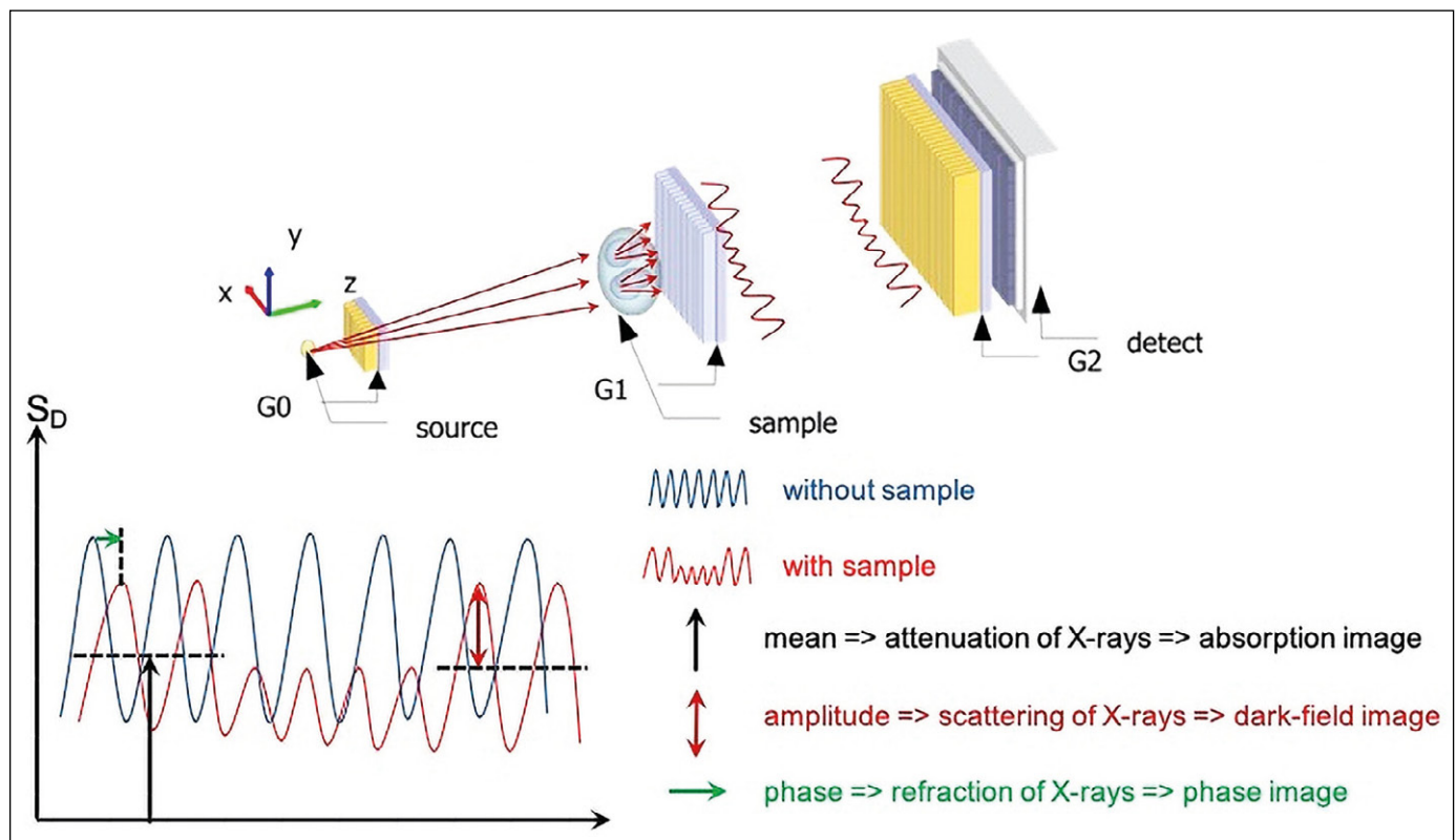
Figure 2. Dark-field imaging (DFI): Talbot-Lau interferometer setup.
