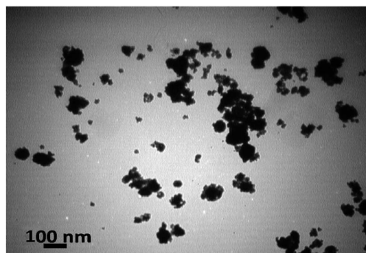
Fig. 3 The TEM image of synthesized NiFe 2 O 4 @SiO 2 @glucose amine.
