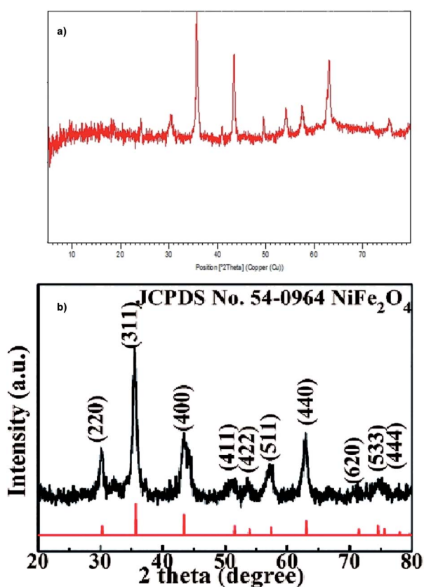
Fig. 2 The XRD of (a) NiFe 2 O 4 @SiO 2 @glucose amine and (b) NiFe 2 O 4 .
