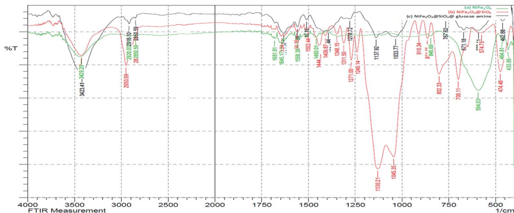
Fig. 1 FT-IR spectra of (a) NiFe 2 O 4 , (b) NiFe 2 O 4 @SiO 2 , (c) NiFe 2 O 4 @SiO 2 @glucose amine.
