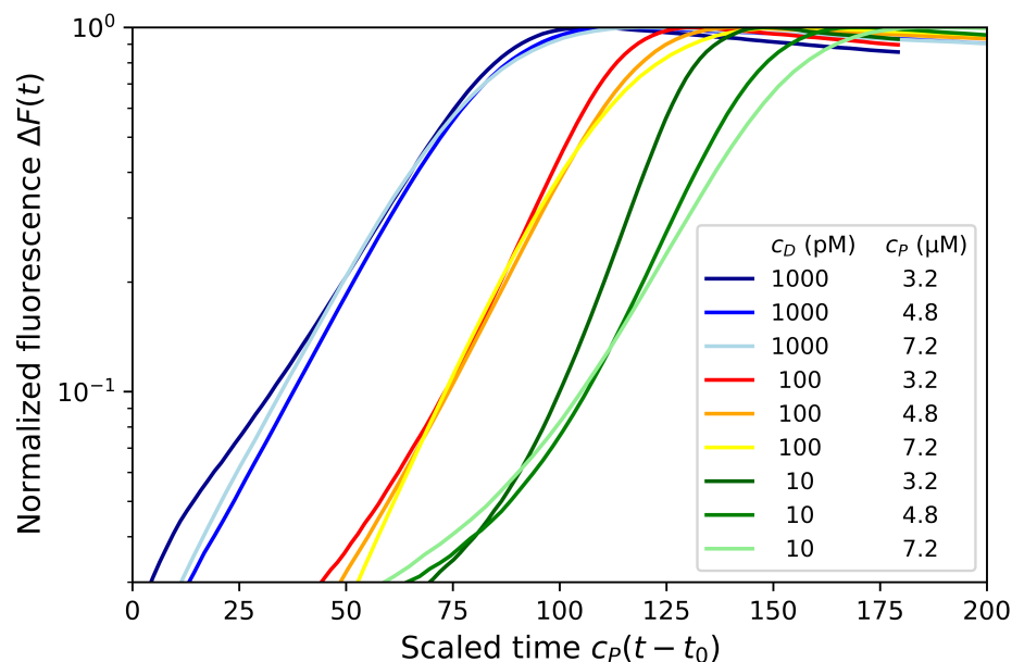
Figure 3. Normalized fluorescence \Delta F in logarithmic scale on the y-axis as function of scaled time c_P(t - t_0) (in \mu\text{M}\cdot\text{min} ) for three concentration of primers ( c_P = 3.2, 4.8, 7.2 \mu\text{M} ) and three MD dumbbell concentrations c_D = 1000, 100, 10 pM.
