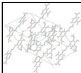
Fig. 2. The molecular packing of the title compound, Hydrogen bonds are shown as dashed lines. H atoms not involved in hydrogen bondings have been omitted for clarity.
