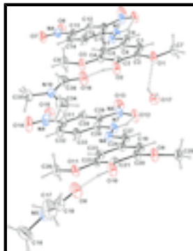
Fig. 1. The asymmetric unit of (I) with the atom-labelling scheme. Displacement ellipsoids are drawn at the 30% probability level. H atoms are represented as small spheres of arbitrary radii. Hydrogen bonds are shown as dashed lines.
