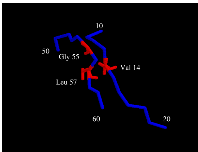
Figure 2 Position of Gly 55 and Leu 57, near Val 14.
