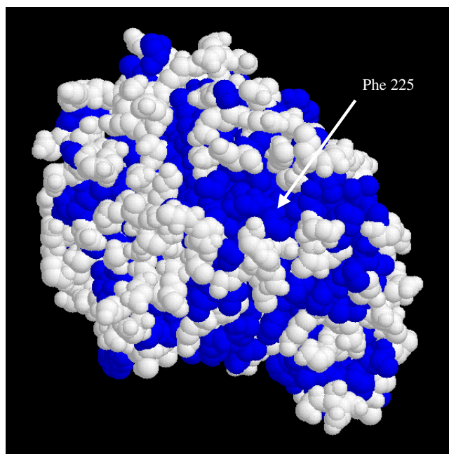
Figure 4 Position of Phe 225 inside an hydrophobic area at the surface of the protein. (hydrophobic residues have been colored in blue).
