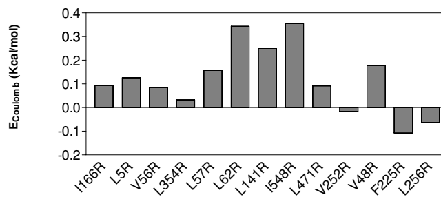
Figure 5 Electrostatic stabilization expected for the charge addition according to the Coulomb's Law ( E = q_1q_2/Dr ) with a dielectric constant of 80 by summing the interactions of the new charge with all the other charges of the protein.
