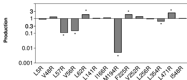
Figure 1 Effect of replacement of hydrophobic residues at the surface by arginine on relative production. Ratio of production represents the relative production of each mutant.
