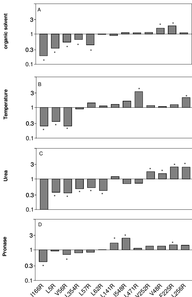
Figure 3 Effect of replacement of hydrophobic residues at the surface by arginine on relative stability. For each mutation, ratio of t_{50} ( t_{50} mutant/ t_{50} wild type) was calculated for each denaturation agent. * indicates a significant difference with the wild type protein with P < 0.05 . Mutations are arranged from the less to the more stable, considering a mean stability for the four parameters analyzed.
