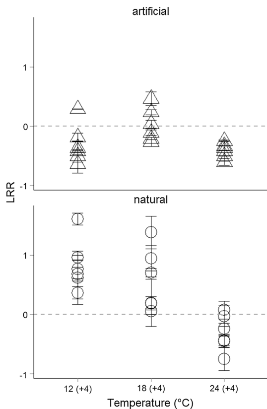
Fig. 3 Log response ratio of chlorophyll a concentrations. Log response ratio (LRR) calculated as the log ratio of chlorophyll a concentrations after pulsed disturbance vs pressed disturbance of natural ( open dots ) and artificial ( open triangles ) communities at different temperatures. Data are shown as mean ( \pm SE) for each site. The dashed line indicates no change in chlorophyll a concentrations; above the dashed line the chlorophyll a concentrations were higher after pulse, below the dashed line higher after press disturbance
