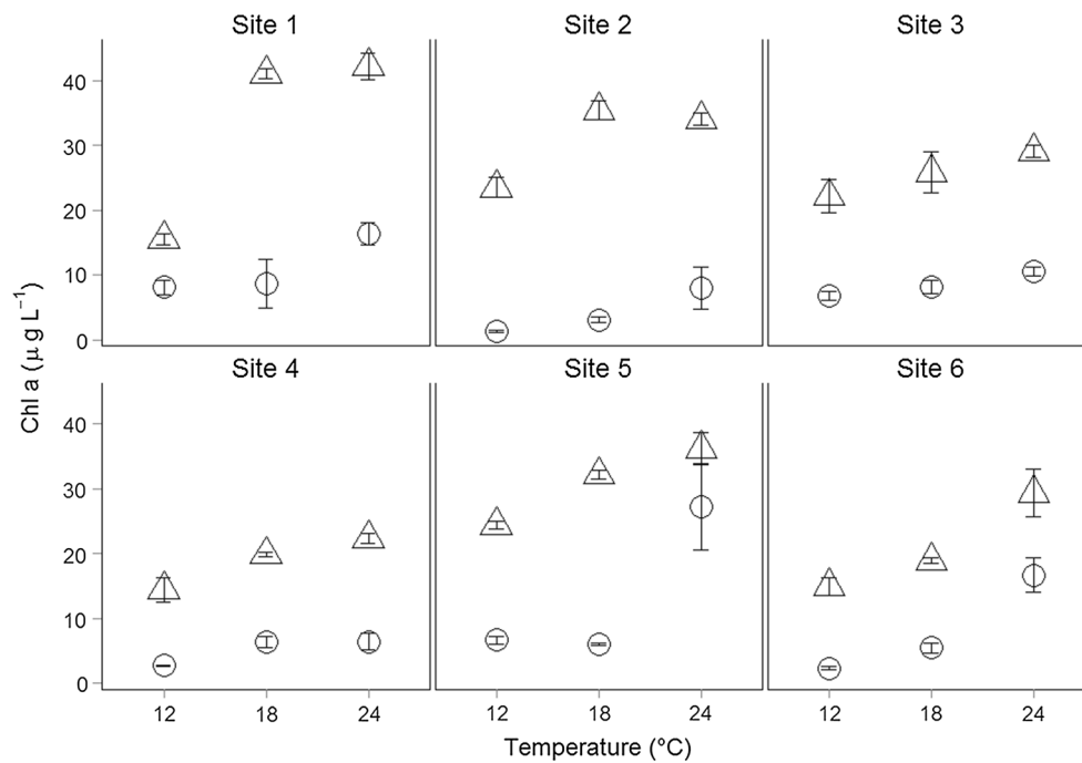
Fig. 1 Phytoplankton biomass after press disturbance. Chlorophyll a concentrations ( \mu\text{g L}^{-1} ) at three temperature levels (12, 18, and 24 °C) for natural ( open dots ) and artificial ( open triangles ) communities after press disturbance (phase I). Data are shown as mean
