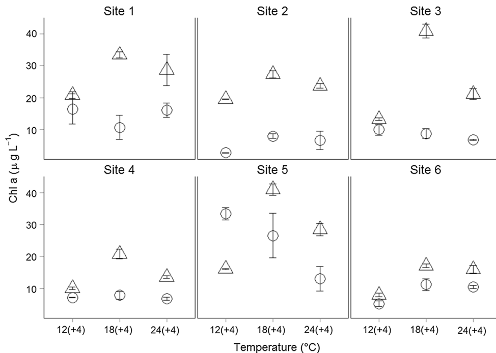
Fig. 2 Phytoplankton biomass after pulse disturbance. Chlorophyll a concentrations ( \mu\text{g L}^{-1} ) at three temperature levels (12(+4), 18(+4), and 24(+4) ^{\circ}\text{C} ) for natural (open dots) and artificial (open triangles) communities after pulse disturbance (phase II). Data are shown as mean ( \pm SE)
