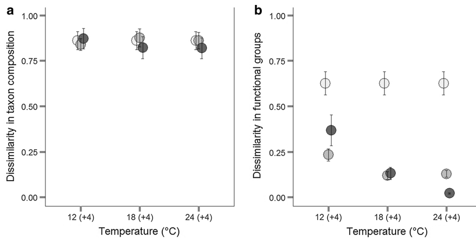
Fig. 5 Dissimilarity between sites. Mean ( \pm SE) dissimilarity (Bray–Curtis) between the different sites was calculated based on species composition ( a ) and functional groups composition ( b ) for the most abundant taxonomic groups (diatoms, green algae, cryptophytes, chrysophytes, cyanobacteria, and dinoflagellates). Dissimilarity was
