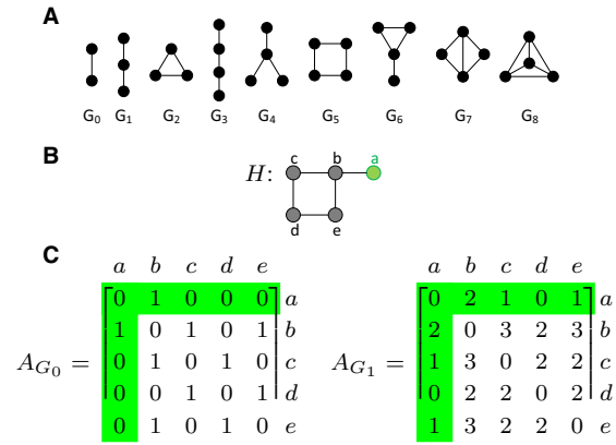
Fig. 1. An illustration of graphlets and graphlet adjacencies. Node a is highlighted throughout. (A) All graphlets with up to four nodes, labeled G_0 to G_8 . (B) Example network H . (C) The graphlet adjacency matrices A_{G_0} and A_{G_1} for graphlets G_0 and G_1 of the example network H , shown in panel (B). The off-diagonal elements correspond to the number of times two nodes touch a given graphlet together. A_{G_0}(a, b) = 1 , as a and b form G_0 once. A_{G_1}(a, b) = 2 , as a and b form G_1 twice, via paths a-b-c and a-b-e . This figure is adapted from Fig. 1 in Windels et al. (2019)
