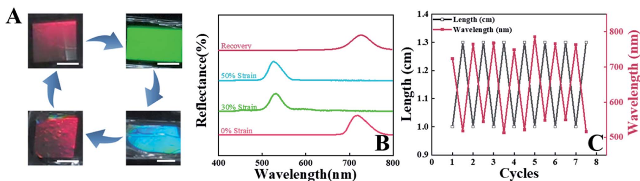
Fig. 2 The evolution of structural colors at a viewing angle of 27^\circ during uniaxial tension along direction A and recovery (A). (B) shows the corresponding reflection spectrum during deformation and recovery. (C) The cycling stability during deformation/recovery with a strain of 30%. The dimension of each color square is 0.5 cm.
