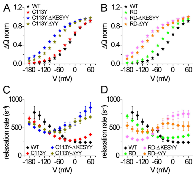
Figure 9. \Delta Y Y and \Delta K E S Y Y truncations shift ouabain-sensitive transient charge movements to more negative potentials and accelerate charge relaxation at positive potentials. (A and B) Charge-voltage distributions determined from OFF voltage steps (as for closed symbols in Fig. 8 [D and H]) were normalized by their estimated amplitude from fits ( Q_{\max} - Q_{\min} , 12.1 nC and 5.4 nC, respectively, for Fig. 8 [D and H]) and were averaged. V_{0.5} and z_1 values for each pump type averaged as follows: WT (black), -16 \pm 1 mV and 0.93 \pm 0.03 , n = 3 ; C113Y (red), -26 \pm 1 mV and 0.70 \pm 0.01 , n = 13 ; RD (green), -44 \pm 1 mV and 0.74 \pm 0.02 , n = 12 ; C113Y- \Delta K E S Y Y (blue), -96 \pm 2 mV and 0.62 \pm 0.05 , n = 7 ; C113Y- \Delta Y Y (olive), -75 \pm 1 mV and 0.67 \pm 0.01 , n = 5 ; RD- \Delta K E S Y Y (magenta), -114 \pm 2 mV and 0.59 \pm 0.02 , n = 11 ; RD- \Delta Y Y (orange), -95 \pm 2 mV and 0.60 \pm 0.02 , n = 5 . (C and D) Single exponential fits to the decay time courses of the transient current elicited by the ON voltage steps (e.g., Fig. 8 C, red lines) gave relaxation rates of the slow components of charge movement; their mean values are plotted against voltage in C and D. Error bars represent SEM.
