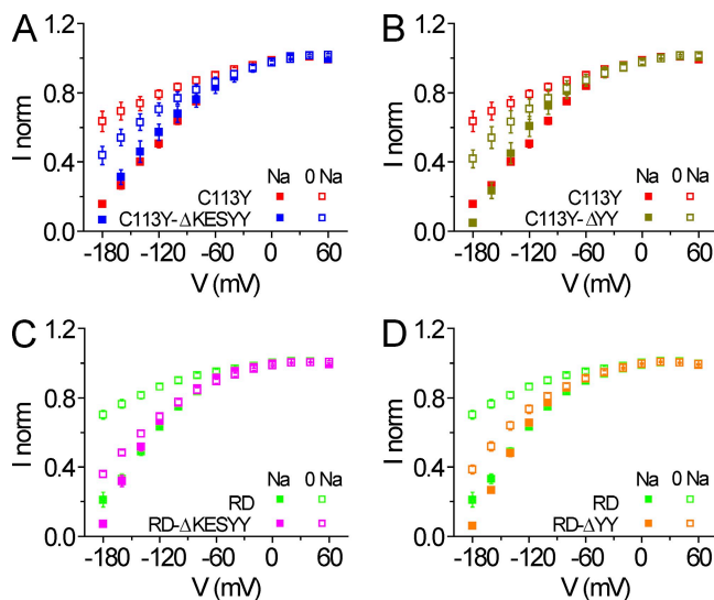
Figure 6. Diminished difference between 125 mM and 0 mM Nao at large negative potentials in \Delta YY and \Delta KESYY truncated Na/K pumps. (A–D) Mean ouabain-sensitive outward Na/K pump currents (normalized as in Fig. 3 D; mean \pm SEM of 6–12 oocytes from at least two frogs) at 15 mM [Ko] and 0 mM Nao (open squares) or 125 mM Nao (closed squares) for \Delta KESYY (A and C) and \Delta YY (B and D) truncated pumps are shown superimposed on the corresponding I-V plots for the parent C113Y (A and B) and RD (C and D) pumps: (A) C113Y (red) and C113Y- \Delta KESYY (blue); (B) C113Y (red) and C113Y- \Delta YY (olive); (C) RD (green) and RD- \Delta KESYY (magenta); (D) RD (green) and RD- \Delta YY (orange). Error bars represent SEM.
