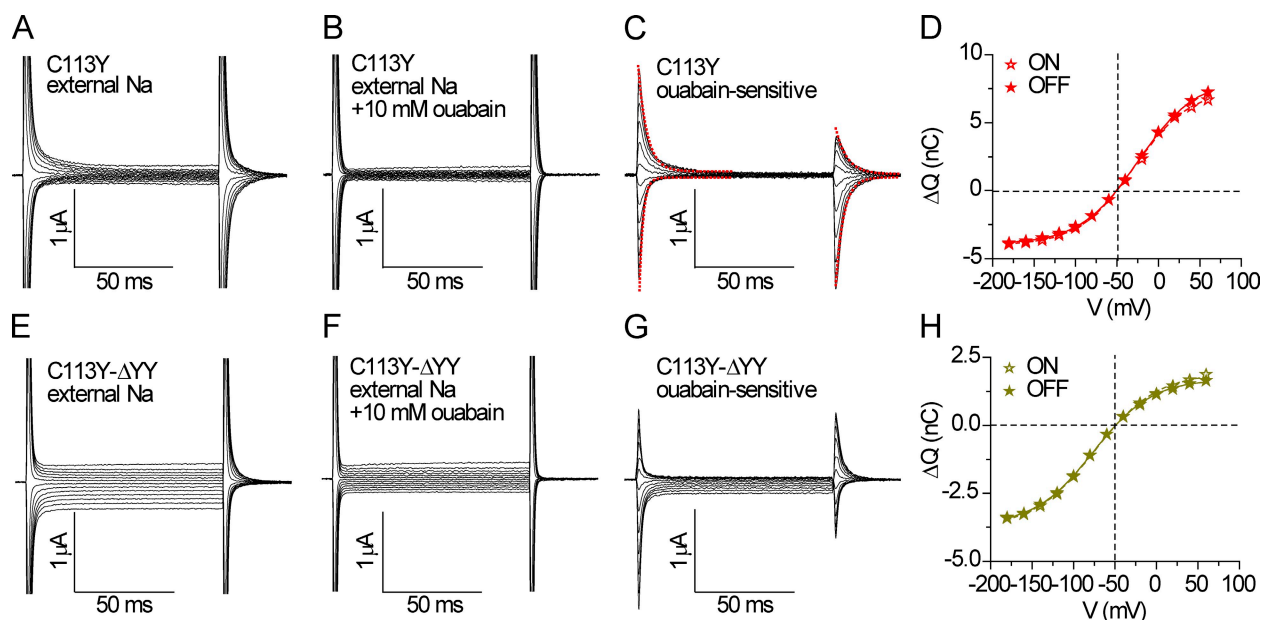
Figure 8. Representative ouabain-sensitive pre-steady-state currents under Na/Na exchange conditions for C113Y and C113Y- \Delta YY pumps. (A–D) C113Y pumps; (E–H) C113Y- \Delta YY pumps. Superimposed current records obtained in 125 mM Na o before (A, C113Y; E, C113Y- \Delta YY) and after (B, C113Y; F, C113Y- \Delta YY) adding 10 mM ouabain. Ouabain-sensitive transient currents determined by direct subtraction of the records in A and B and in E and F, respectively, are shown in C for C113Y and in G for C113Y- \Delta YY Na/K pumps (red lines in C show single exponential fits to ON and OFF transient currents elicited by steps to 60 mV and -180 mV for relaxation rate estimates of Fig. 9 [C and D]). Pre-steady-state charge was obtained directly as the time integral of the transient currents (C and G) at the ON and OFF voltage steps after baseline subtraction of any steady current. (D and H) The charge–voltage distributions were fit with the Boltzmann relation
