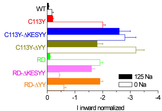
Figure 4. Comparison of the magnitude of ouabain-sensitive inward current in each pump type at -180 \text{ mV} ( -160 \text{ mV} for WT) in the absence or presence of 125 mM Nao after normalization by the ouabain-sensitive pump current activated by 15 mM [Ko] at the -50 \text{ mV} holding potential in the same oocyte and [Nao] to allow for differences in expression. Open bars, absence of 125 mM Nao; closed bars, presence of 125 mM Nao. Mean values are -0.04 \pm 0.02 , n = 4 , in 125 mM Nao and -0.17 \pm 0.05 , n = 4 , in 0 mM Nao for WT Na/K pumps (black); -0.20 \pm 0.03 , n = 8 , in 125 mM Nao and -2.0 \pm 0.1 , n = 8 , in 0 mM Nao for C113Y (red); -2.6 \pm 0.4 , n = 5 , in 125 mM Nao and -2.8 \pm 0.4 , n = 5 , in 0 mM Nao for C113Y- \Delta KESYY (blue); -1.8 \pm 0.2 , n = 6 , in 125 mM Nao and -3.2 \pm 0.6 , n = 6 , in 0 mM Nao for C113Y- \Delta YY (olive); -0.10 \pm 0.02 , n = 7 , in 125 mM Nao and -1.9 \pm 0.1 , n = 7 , in 0 mM Nao for RD (green); -1.6 \pm 0.1 , n = 8 , in 125 mM Nao and -0.43 \pm 0.03 , n = 8 , in 0 mM Nao for RD- \Delta KESYY (magenta); and -1.9 \pm 0.1 , n = 7 , in 125 mM Nao and -0.60 \pm 0.08 , n = 7 , in 0 mM Nao for RD- \Delta YY (orange). Error bars represent SEM.
