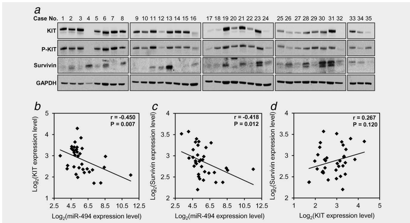
Figure 3. Relationships between the expression of survivin, miR-494 and KIT in 35 GIST tissues. (a) The expression levels of KIT, P-KIT, survivin and GAPDH were measured in 35 GIST tissues using western blot analysis. (b–d) Statistical correlation analysis was performed for the expression of KIT and miR-494 (Pearson's correlation coefficient, r = -0.450 , p = 0.007 ), the expression of survivin and miR-494 (Pearson's correlation coefficient, r = -0.418 , p = 0.012 ) and the expression of KIT and survivin (Pearson's correlation coefficient, r = 0.267 , p = 0.120 ).
