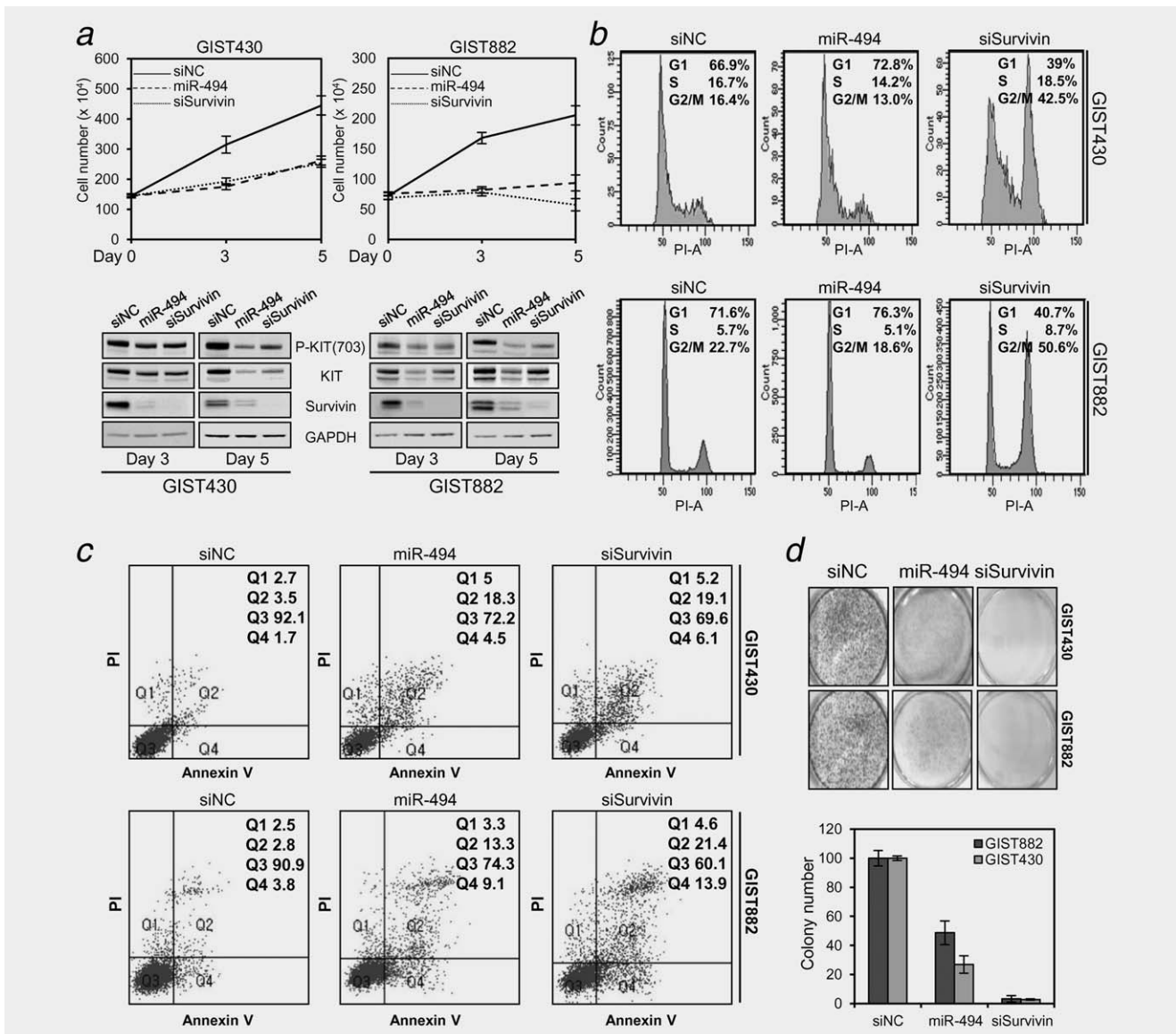
Figure 4. Downregulation of survivin inhibits proliferation of GIST cells via the perturbation of the cell cycle. (a) Proliferation of GIST430 and GIST882 cells after exposure to miR-494 or siSurvivin was measured by manually counting cells at 3- and 5-day post-exposure. Knock-down efficiency of miR-494 and survivin was confirmed using western blot analysis of KIT and survivin. (b, c) Cell-cycle (propidium iodide staining) and apoptosis (Anexin and propidium iodide staining) analysis in GIST430 and GIST882 cells were performed after exposure to miR-494 or siSurvivin. (d) Colony formation of GIST430 and GIST882 cells was evaluated after miR-494 or siSurvivin treatment. Two weeks after seeding 40,000 cells of GIST430 and GIST882, colonies were stained using crystal violet and were counted using a Colony V1.1.
