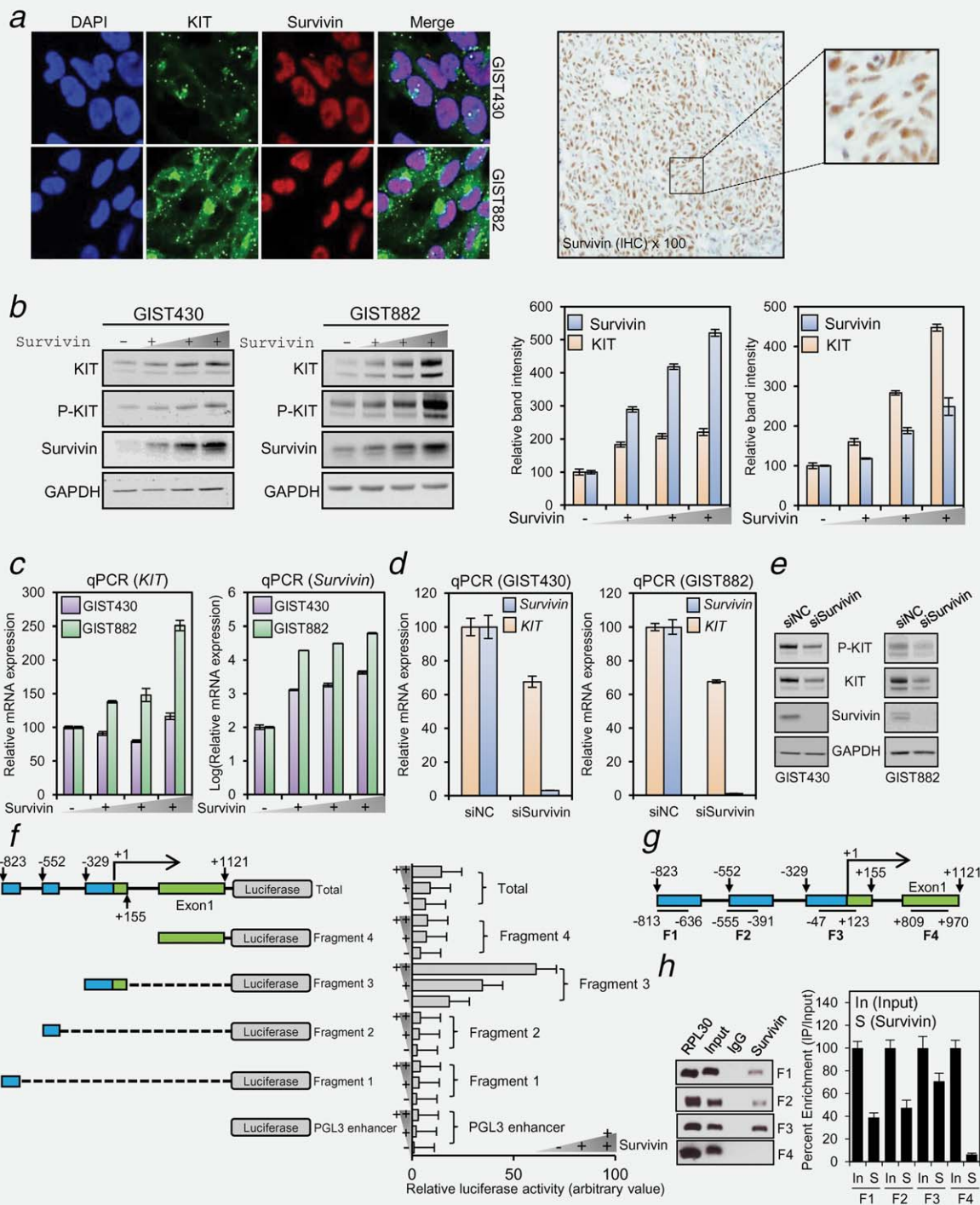
Figure 6. Survivin binds to a specific region of the KIT promoter and induces KIT expression at the transcription level. (a) The localization of KIT and survivin was examined using GIST430 and GIST882 cells and immunofluorescence microscopic analysis (left panel). The nuclear localization of survivin was examined by immunohistochemistry in a representative GIST tissue (right panel). (b, c) The changes in expression of KIT mRNA and protein were evaluated using qPCR and western blot in GIST430 and GIST882 cells transfected with gradually increasing amount of survivin plasmids. (d, e) Expression of KIT mRNA and protein were measured after siSurvivin treatment. (f) To map a specific region of KIT promoter bound by survivin, various KIT promoter fragments conjugated with Firefly luciferase (five different fragments, including the full-length promoter) were constructed, and dual luciferase assay was performed 48 hr after transfection of each construct with survivin expression vector into HeLa cells. The schematic map of the vectors is presented on the left panel and the relative luciferase activity results are presented on the right panel. The KIT promoter region was obtained from bioinformatic software (MethPrimer). To determine the relative luciferase activity, the Firefly luciferase activity was normalized based on the Renilla luciferase activity. (g) Chromatin immunoprecipitation assay performed using anti-survivin, anti-histone H3 and normal rabbit IgG antibodies. (h) Enrichment of the survivin-binding DNA fragment in the KIT promoter region was evaluated by semi-qPCR. In the positive control sample, binding of histone H3 to RPL30 exon 3 was evaluated (left panel). Densitometric analysis of the intensity of semi-qPCR assay bands (right panel).
