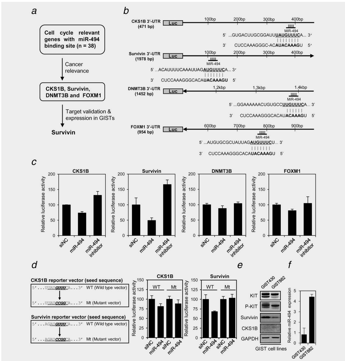
Figure 2. MiR-494 directly regulates survivin, which is universally overexpressed in GIST cells. (a) Putative novel miR-494 target genes were selected ( CKS1B , survivin , DNMT3B and FOXM1 ) based on previous reports and cancer relevance. Survivin was selected after target validation assay, and endogenous protein expression level, results. (b, c) The reporter vector was constructed by conjugating Renilla luciferase with a Target-Scan predicted miR-494 binding site in each 3'-UTR of CKS1B , survivin , DNMT3B and FOXM1 . Each reporter vector with siNC, miR-494 or miR-494 inhibitor was transfected into HeLa cells. Dual luciferase assays were performed by measuring Renilla and Firefly luciferase activity at 48 hr post-transfection. (d) Mutant reporter vectors for CKS1B and survivin were further constructed by substituting seed match sequences of miR-494 (GTTT->CCGG). After transfection of the wild-type reporter vector (WT) and mutant reporter vector (Mt) with siNC or miR-494, a dual luciferase assay was performed. WT denotes the wild-type vector with the original binding site of miR-494. Mt denotes the mutant vector with a mutated binding site of mR-494. To determine the relative luciferase activity, the Renilla luciferase activity was normalized based on the Firefly luciferase activity. (e, f) Endogenous survivin , CKS1B and miR-494 expression analyzed by western blotting and qPCR analysis, respectively, in GIST430 and GIST882 cells.
