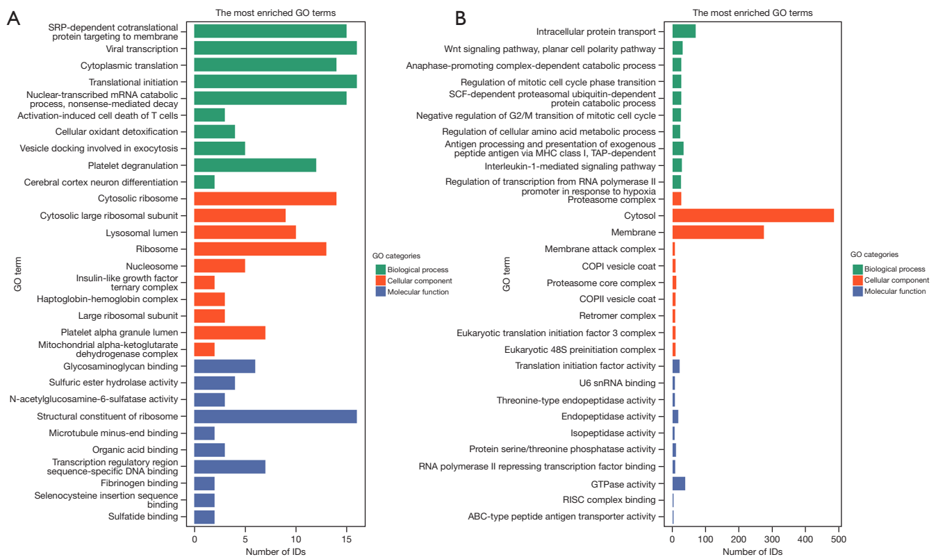
Figure 2 The GO analyses results of the MML/MNML group (A) and the BML/BNML group (B). GO, Gene Ontology; MML, malignant mass-like; MNML, malignant non-mass-like; BML, benign mass-like; BNML, benign non-mass-like.
