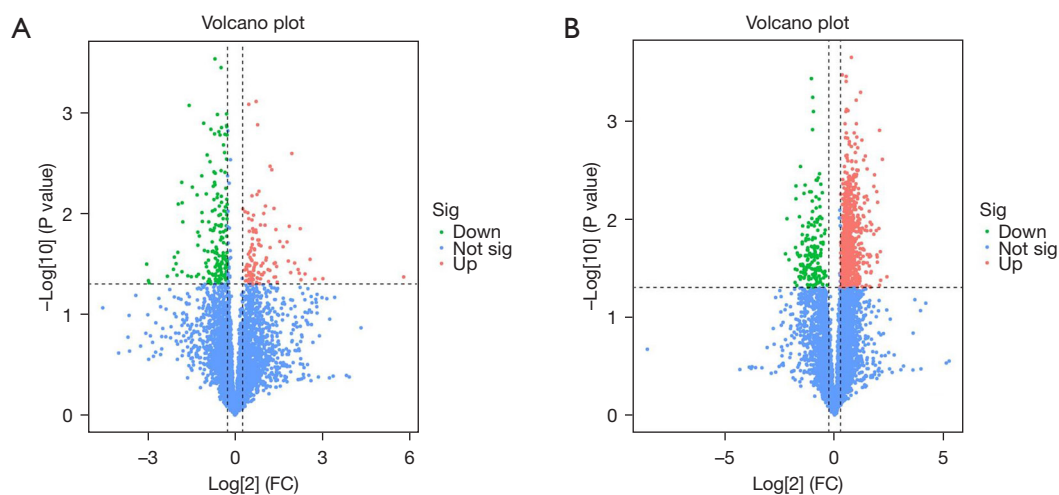
Figure 1 Quantitative volcano plot of differentially expressed proteins in each group. (A) The quantitative volcano plot of differentially expressed proteins in the MML/MNML group; (B) the quantitative volcano plot of differentially expressed proteins in the BML/BNML group. FC, fold change; MML, malignant mass-like; MNML, malignant non-mass-like; BML, benign mass-like; BNML, benign non-mass-like.
