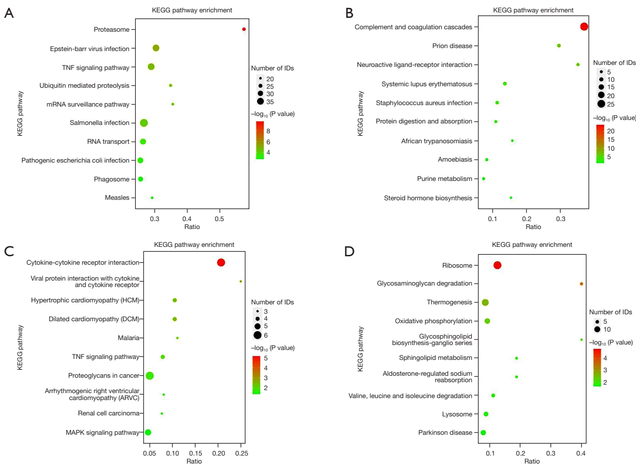
Figure 3 The top 10 up- and down-regulated protein enrichment KEGG pathways in the MML/MNML (A,B) and BML/BNML (C,D) groups. KEGG, Kyoto Encyclopedia of Genes and Genomes; TNF, tumor necrosis factor; MML, malignant mass-like; MNML, malignant non-mass-like; BML, benign mass-like; BNML, benign non-mass-like.
