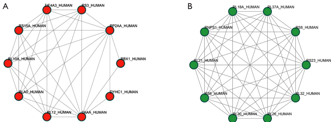
Figure 4 The specific linkage results of the top 10 key proteins in the PPI network in the MML/MNML (A) and the BML/BNML (B) groups. PPI, protein-protein interaction; MML, malignant mass-like; MNML, malignant non-mass-like; BML, benign mass-like; BNML, benign non-mass-like.
