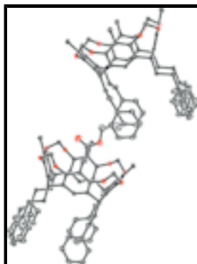
Fig. 3. The relative orientation of the feet in neighbouring resorcin[4]arene units. Displacement ellipsoids are drawn at the 10% probability level. The inclusion of the ethyl acetate solvent molecule between aromatic groups is shown. H atoms are omitted.
