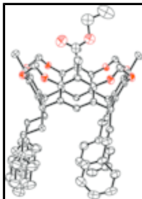
Fig. 2. The molecular structure with displacement ellipsoids drawn at the 50% probability level. H atoms are omitted. The "bowl" shape of the molecule is evident, with the ethyl acetate molecule present as a guest in the molecular cavity.
