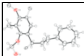
Fig. 1. A view of one quarter of the cyclic tetramer. Displacement ellipsoids are drawn at the 50% probability level and H atoms are shown as spheres of arbitrary radii. Dashed bonds indicate links to the neighbouring units.
