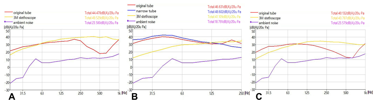
Figure 4 Comparison of the frequency spectra of 3 M Littmann lightweight stethoscopes and cylindrical tube stethoscopes. (A) Pulmonary auscultation. (B) Cardiac auscultation. (C) Intestinal auscultation.
