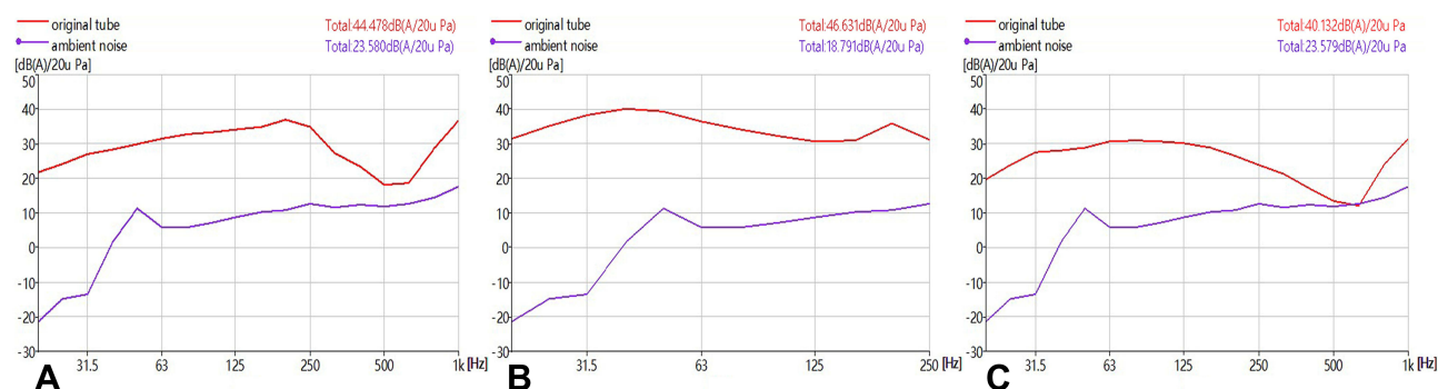
Figure 2 Frequency spectra of sound pressure levels measured using the original stethoscope. (A) Measured at the triangle of auscultation of the lungs. (B) measured at the apex area of the heart. (C) measured at McBurney's point of the intestines.
