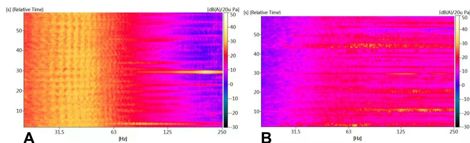
Figure 5 Spectrogram of heart sound signals of all ten volunteers measured using stethoscope (A) the cylindrical tube stethoscope. (B) the 3 M stethoscope.
