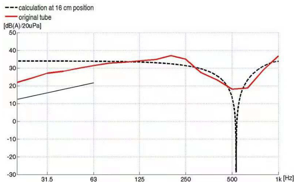
Figure 3 The measured and calculated pulmonary sound pressure levels of the cylindrical tube stethoscope.
