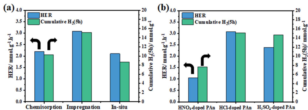
Fig. 9 The initial and cumulative (5 h) hydrogen evolution rate of (a) TiO 2 @5PAN composites fabricated by chemisorption, in situ polymerization, and impregnation methods and (b) TiO 2 @5PAN composites modified with various counterions, NO 3 - , SO 4 2- , and Cl - .
