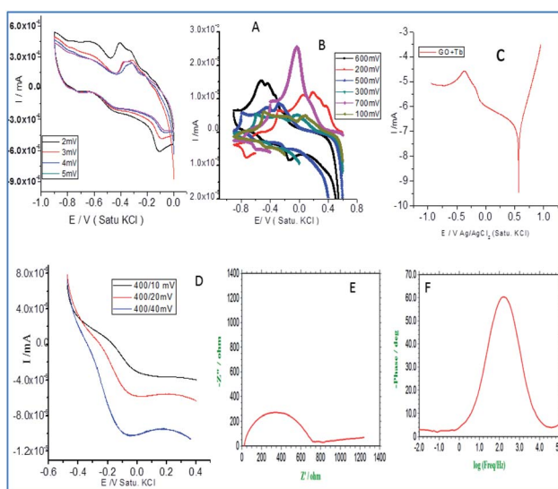
Fig. 3 Electrochemical studies of Tb-functionalized graphene oxide: (A and B) cyclic voltammety (C) Tafel curve (D) linear sweep voltammety (E) impedance Nyquist (F) impedance phase.
