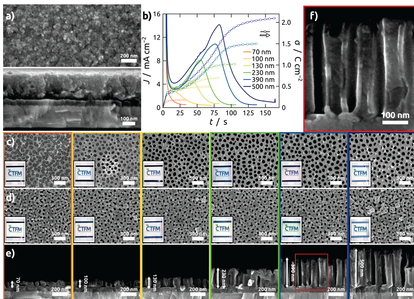
Figure 2. Anodization of Al metal evaporated on a transparent electrode. (a) SEM top view (upper image) and cross section (lower image) of a 200-nm aluminum layer on a glass/ITO/TiO 2 substrate. (b) Anodization current density and surface charge density plotted against anodization time for all AAO pore lengths produced here. (c–e) SEM micrographs of samples with pore lengths of 70, 100, 130, 230, 390, and 500 nm (from left to right) in three situations: (c) in top view after anodization and subsequent pore widening, (d) in top view after further TiO 2 ALD (10 nm) and annealing at 500 °C for 1 h, and (e) in cross section after these steps. The red frame in (e) is enlarged in (f).
