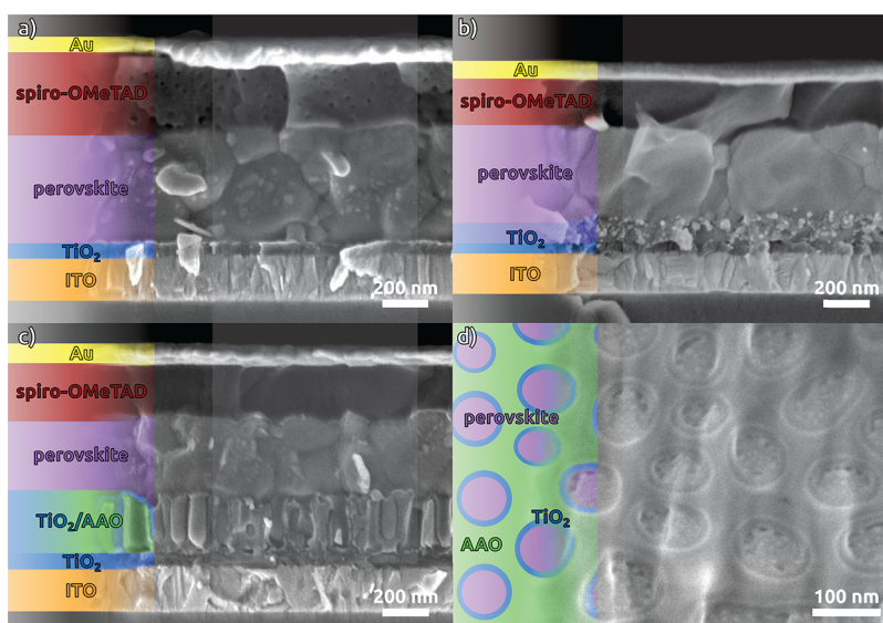
Figure 4. Cross-section of the three different geometries: (a) planar, (b) mesoporous, and (c) AAO pores with the basic device structure of glass/ITO/c-TiO 2 /ALD or mp-TiO 2 /Cs 0.5 (FA 0.83 MA 0.17 ) 0.95 Pb(I 0.83 Br 0.17 ) 3 /spiro-OMeTAD/Au. (d) Filled AAO pores cut by ion milling of a sample with 390 nm pore length.
