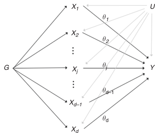
Fig. 2 Directed acyclic graph of instrumental variable assumptions made in multivariable Mendelian randomization. G = genetic variants, X_j = risk factor j for j = 1, \dots, d , Y = outcome, U = confounders, \theta_j = causal effect of risk factor j .
