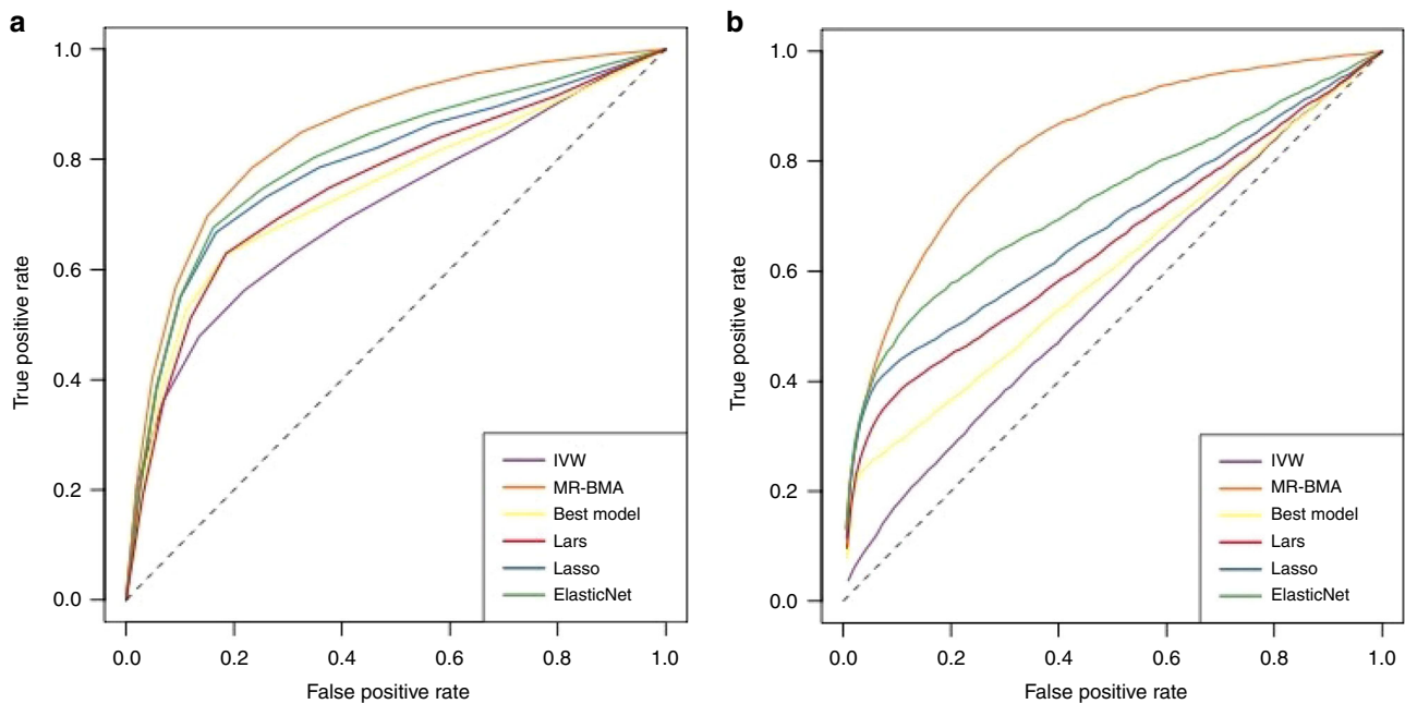
Fig. 3 Receiver operating characteristic (ROC) curve for simulation study on metabolite GWAS. ROC curves plotting the true positive rate against the false positive rate for a a small number of risk factors ( d = 12 ) of which four have true positive effects (Scenario 1, Setting A) and for b a large number of risk factors ( d = 92 ) of which four have true positive effects (Scenario 2, Setting A). Proportion of variance explained ( R^2 ) is set to 0.3.
