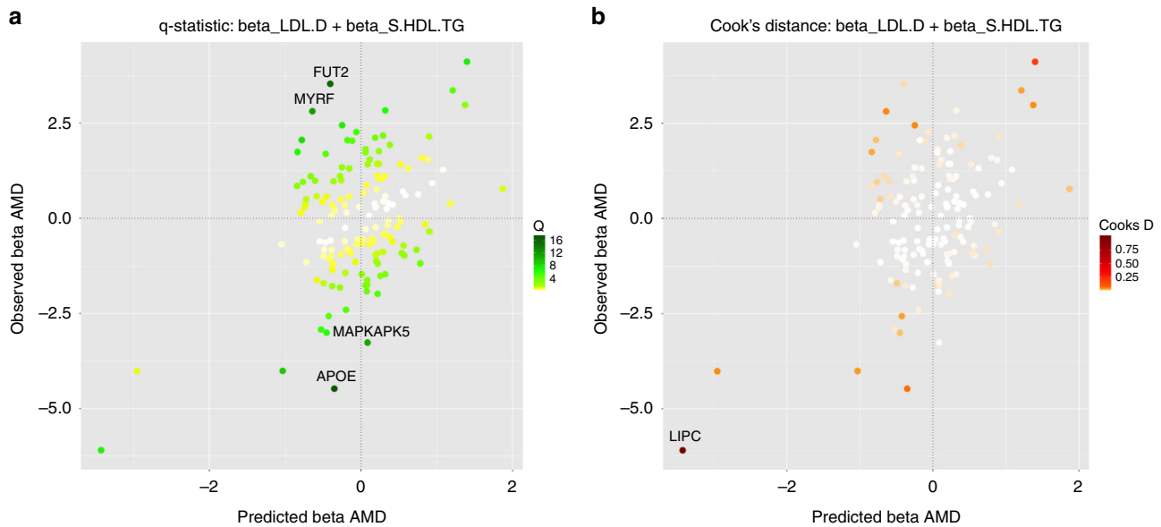
Fig. 4 Diagnostic plots for outliers and influential genetic variants. Plotting the predicted associations with AMD based on the model including LDL.D, and S.HDL.TG (x-axis) against the observed associations with AMD (y-axis) showing all n = 148 genetic variants. This is the highest-ranking model when keeping outlying and influential genetic variants in the analysis. The colour code shows: a the q -statistic for outliers and b Cook's distance for the influential points. Any genetic variant with q -value larger than 10 or Cook's distance larger than the median of the relevant F -distribution is marked by a label indicating the gene region.
