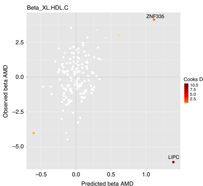
Fig. 5 Diagnostic plot for influential genetic variants. Plotting the predicted associations with AMD based on the model including XL.HDL.C (x-axis) against the observed associations with AMD (y-axis) showing all n = 148 genetic variants, where the colour code shows Cook's distance for the genetic variants. This is the highest-ranking model on omission of outlying and influential genetic variants from the analysis. Note rs26134 in the LIPC gene region which has an anomalous direction of association with AMD risk in contrast to all other genetic variants.
