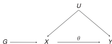
Fig. 1 Directed acyclic graph of instrumental variable assumptions made in univariable Mendelian randomization. G = genetic variant(s), X = risk factor, Y = outcome, U = confounders, \theta = causal effect of interest.
