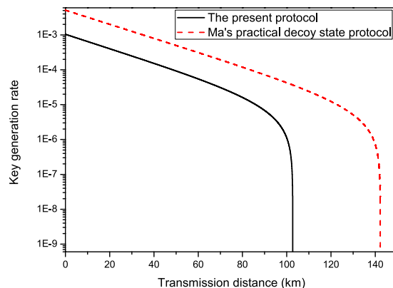
Figure 2. The solid line represents the relation between the key generation rate and the transmission distance of the present protocol. The dash line characterizes the relation between the key generation rate and the transmission distance in ref. 14.
