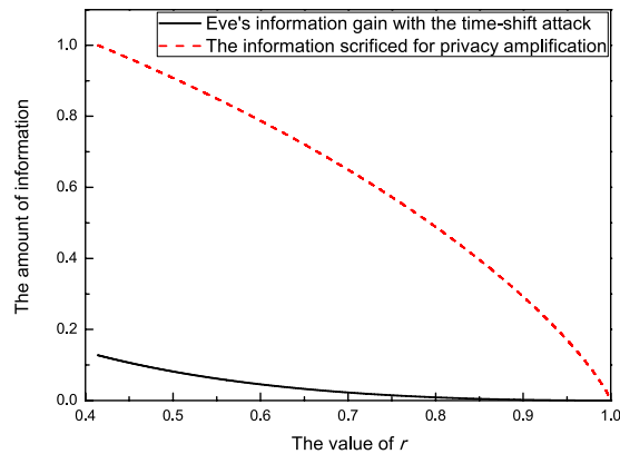
Figure 1. The solid line represents Eve's information gain within her time-shift attack. The dash line represents the amount of information Alice and Bob should sacrifice for PA after Eve's time-shift attack.
