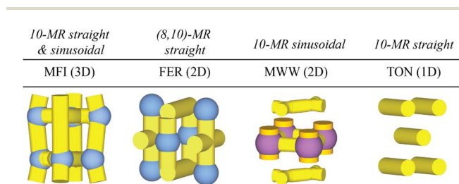
Fig. 1 The project design: mechanism of catalytic cracking of alkanes will be investigated over the following 10-membered ring (MR) zeolites: ZSM-5 (3D MFI topology), FER (2D FER topology), MCM-22 (2D MWW topology), and ZSM-22 (1D TON topology). Typically, 10-MR zeolites provide superior molecular traffic control compared to other MR zeolites. Despite their structural and topological diversity, these zeolites are intriguing for mechanistic investigations in zeolite catalysis. In this context, the zeolite's channels, presented in yellow ( D < 6 Å), are illustrated in italics, while the cages or intersections are depicted in blue ( D \sim 6–8 Å) and purple ( D > 8 Å) spheres. 27
