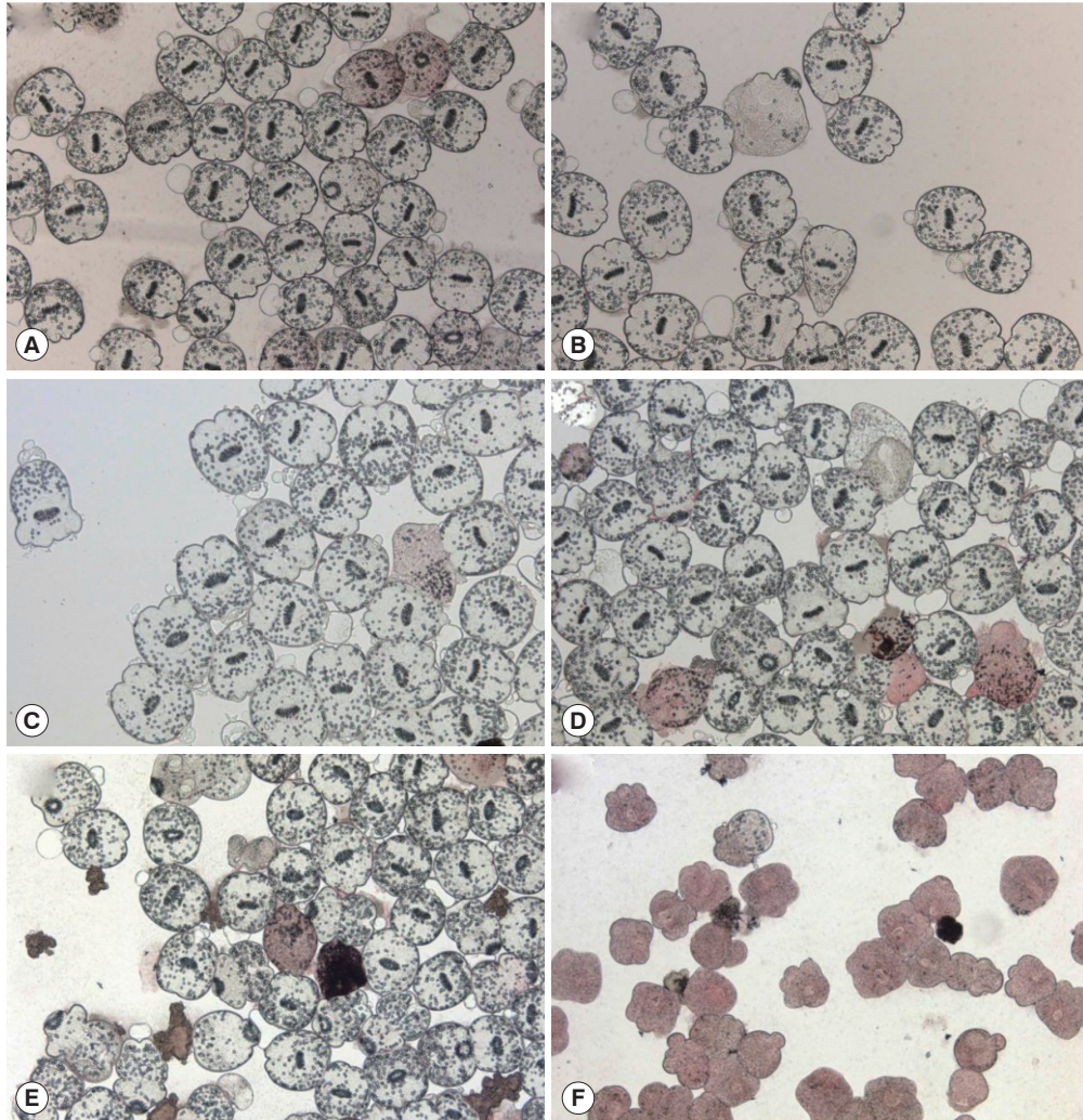
Fig. S1. Protoscolices of E. granulosus treated with drugs in vitro. (A) Protoscolices after 5 days of cultivation under normal (untreated) conditions, or with (B) DMSO, (C) 7.5 \mu M ML3403, (D) 15 \mu M ML3403, (E) 30 \mu M ML3403, and (F) 60 \mu M ML3403.
