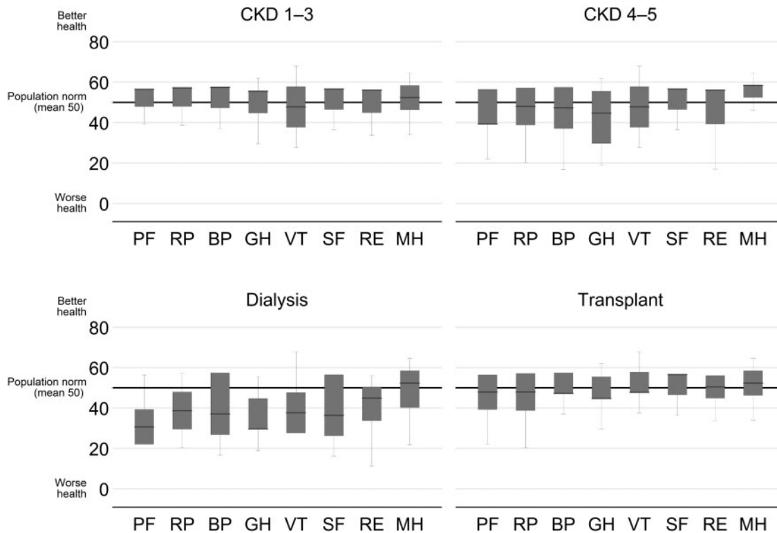
FIGURE 1: Norm-based scoring of the Short Form-12 Health Survey (SF-12) profile. All SF-12 scales are standardized to have a mean of 50 and standard deviation of 10 in the general 1998 US population (range: 0–100). Boxes extend from the 25th to 75th percentiles with the median highlighted; whiskers (vertical lines) extend 1.5 times the interquartile range. PF, physical functioning; RP, role physical; BP, bodily pain; GH, general health; VT, vitality; SF, social functioning; RE, role emotional; MH, mental health.
