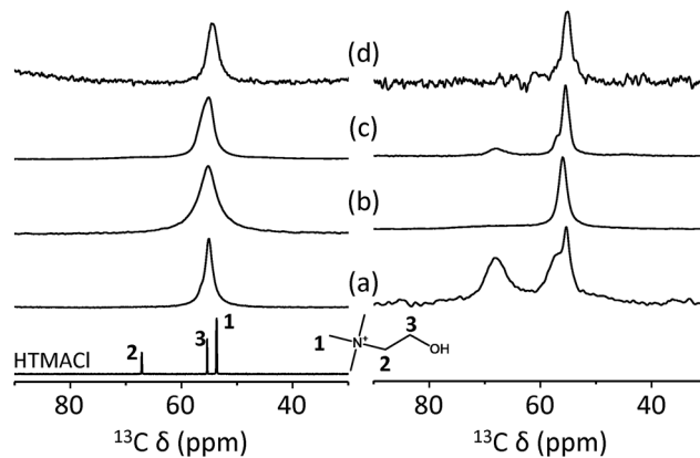
Fig. 4 13 C MAS (left) and 1 H– 13 C CP MAS (right) NMR spectra of the as-made form of (a) UZM-22, (b) PST-10C and (c) ECR-40C and (d) the seven-times Na + -exchanged form of ECR-40C. The 13 C solution NMR spectrum of HTMACl in D 2 O is also given for comparison.
