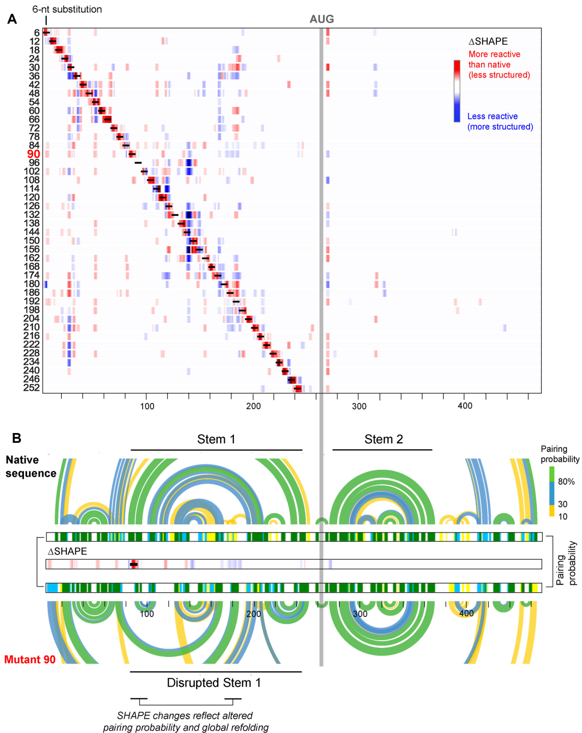
Figure 3. Consequences of local structure-destabilizing mutations across the NM_000295.4 5'-UTR and initial CDS. (A) Heat map of SHAPE reactivity changes—quantified as \Delta SHAPE changes (44)—for each mutant relative to the native sequence transcript. Mutation sites are indicated by black bars; mutants are named by the position of their 3'-most substituted nucleotide. Increases and decreases are shown on a red to blue scale. (B) Arc diagrams, linear pairing probability plots, and \Delta SHAPE (middle) for representative structure-altering mutant (mutant 90) versus native sequence transcript. Site of mutation indicated by black bar.
