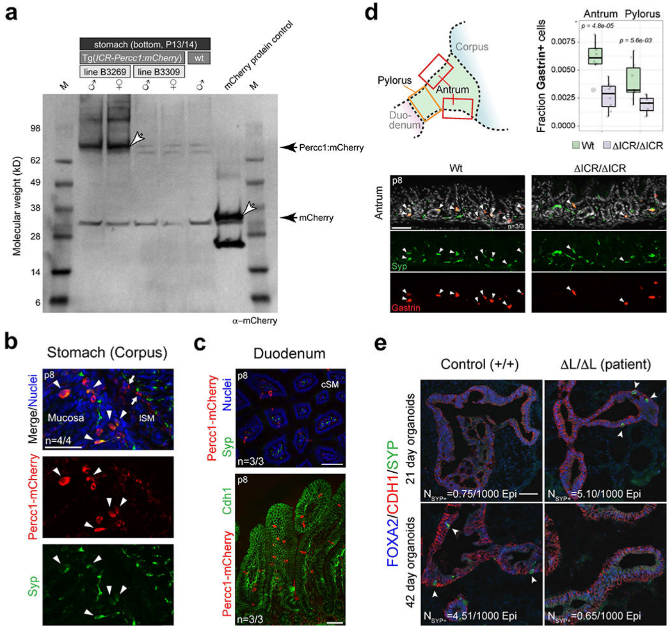
Extended Data Figure 7. Characterization of PERCC1 in mice and patients.
