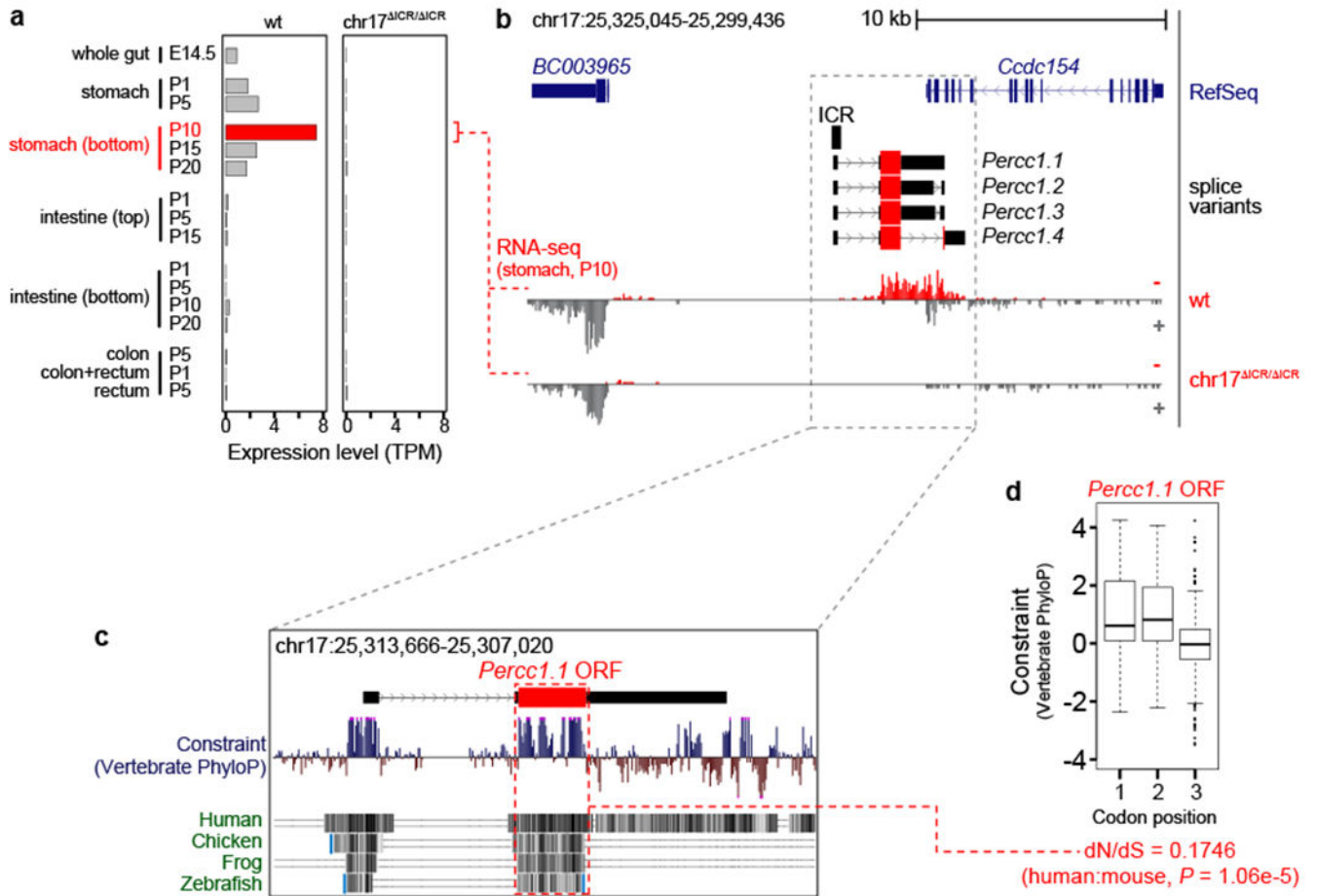
Figure 3. Discovery of a novel gene, Percc1 , flanking the ICR.
