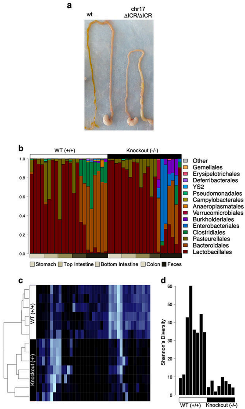
Extended Data Figure 4. Gastrointestinal and microbiome analysis in chr17 ICR/ICR mice. a , Modified intestinal content in wild type (left) compared to chr17 ICR/ICR mice at postnatal day 10 (n=45, right). b,c,d , ICR deletion causes changes in intestinal and fecal microbiome composition. Microbial communities in different intestinal compartments and feces were profiled by 16S rRNA-based sequence profiling. b , Family-level relative abundance profiles of the top fifteen most abundant prokaryotic families for wild type (n=22) and chr17 ICR/ICR (n=21) intestinal and fecal samples, organized by sample type. The most pronounced changes were observed in colon and fecal samples. c , Heatmap of log-
