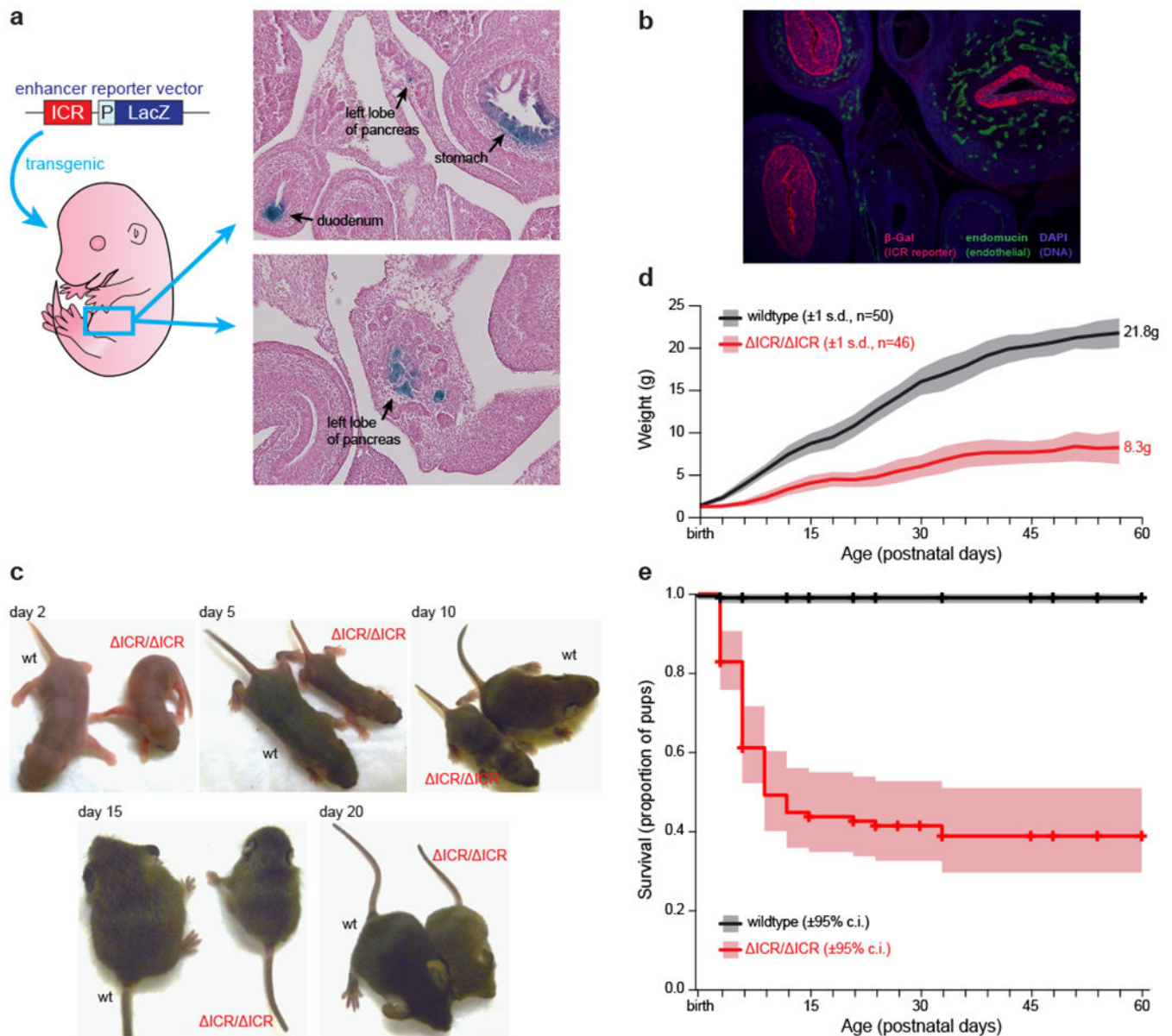
Figure 2. Enhancer activity of the ICR and mouse deletion phenotypes.
