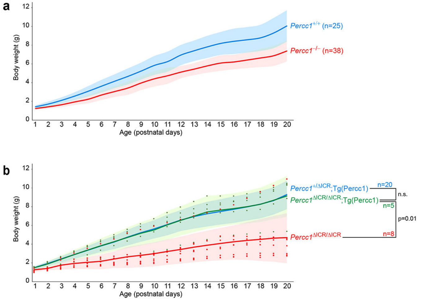
Extended Data Figure 6. Body weight analysis in Percc1 knockout and transgenic mice. a , Percc1 knockout mice have reduced body weight. Percc1 knockout mice (n=38) weight comparison to littermate controls (n=25) (red Percc1 knockouts, blue littermate controls). Lines represent the mean. Shaded areas represent +/- 1SD. Percc1 knockout mice were generated in an FVB/N genetic background. b , Percc1 transgenic rescue of the body weight phenotype found in chr17 ICR/ICR mice. An 8.5kb Percc1 mini gene was constructed (Supp. Table 10) and used to generate a Percc1 mouse line over-expressing PERCC1. Through introduction of this transgene into the chr17 ICR/ICR mouse genetic background, we observed rescue of all the phenotypes found in chr17 ICR/ICR mice including severe body weight reduction. Chr17 ICR/ICR mice were generated in a mixed 129/C57Bl6 background. Center point of lines represent the mean. Shaded areas represent +/- 1SD. P values were determined using a 2-tailed T-test. n.s.= p value 0.8-1.0.
