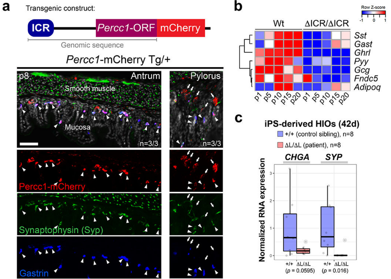
Figure 4: PERCC1 is abundant in G-cells and its genetic disruption impairs gastrointestinal peptide hormone expression and enteroendocrine cell development.
