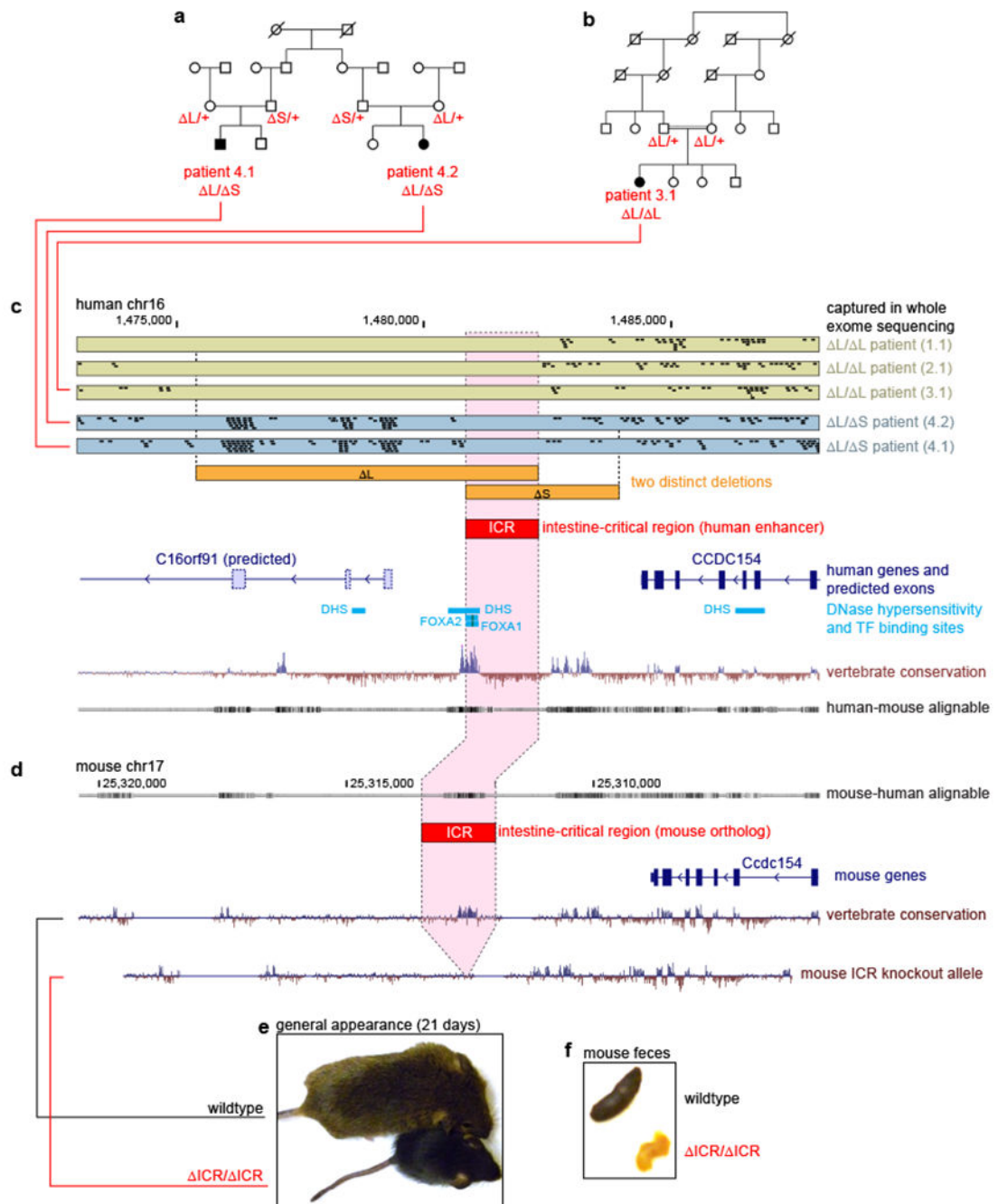
Figure 1. Overview of human and mouse locus and key findings.
