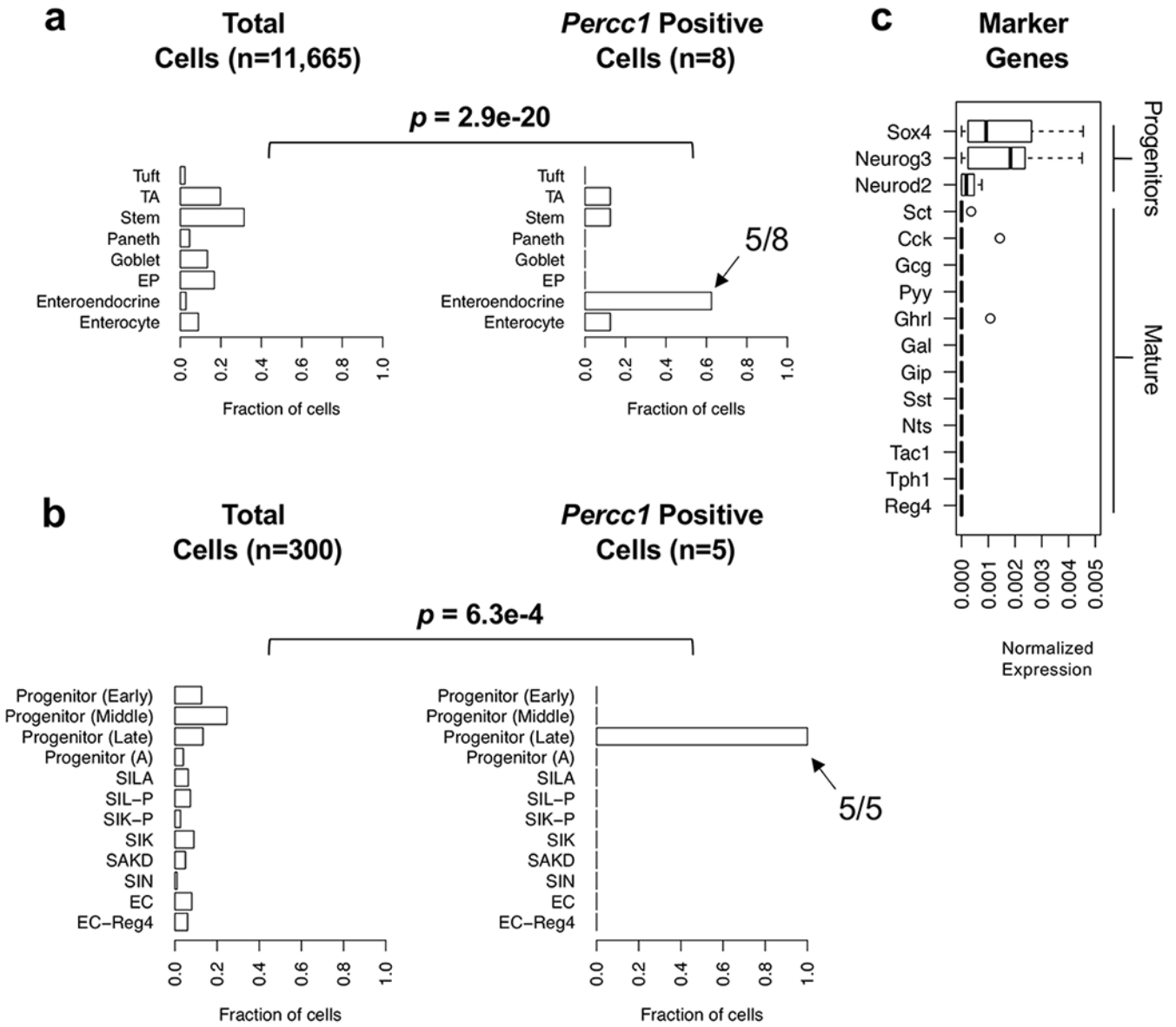
Extended Data Figure 8. Percc1 analysis in mouse intestinal single cell transcriptomes.
