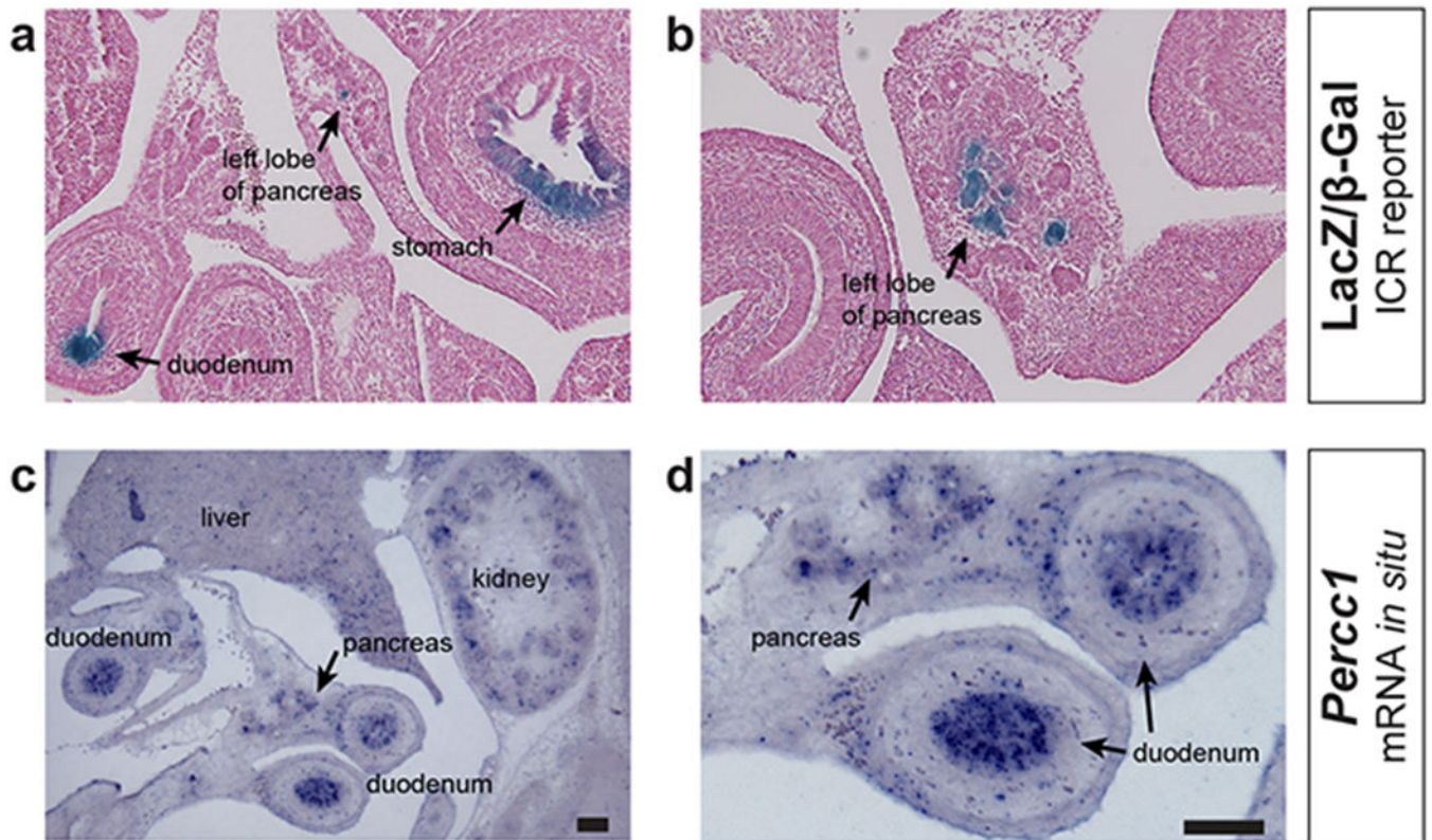
Extended Data Figure 5. Gastrointestinal X-gal ( \beta -gal) staining of ICR-reporter transgenic embryos compared to Percc1 mRNA in situ hybridization.
