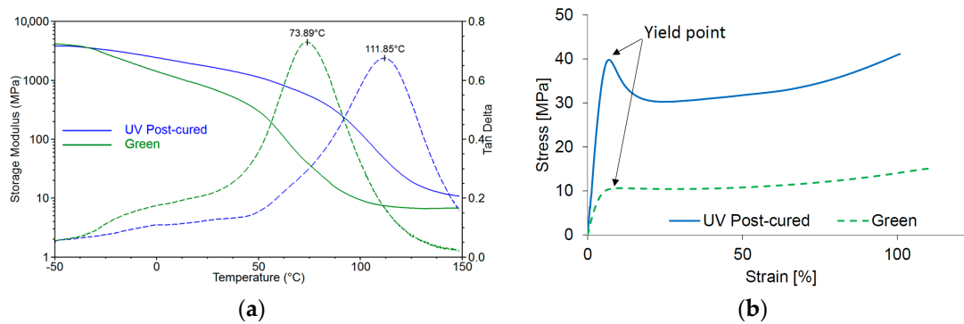
Figure 10. Testing of DLP-printed samples (1.18 wt % TPO-L): (a) Storage modulus (solid line) and the \tan \delta -curve (dashed line) for green and post-cured samples. The peak of the \tan \delta -curve was analyzed; (b) Stress-strain curves from tensile tests. The samples show a yield point, which was used for the analysis.
