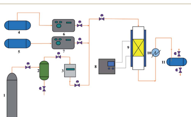
Fig. 1 Experimental setup for the catalytic performance evaluation. 1-N 2 cylinder, 2-desiccator, 3-mass flow controller, 4-naphtha container, 5-methanol container, 6-constant flux pump, 7-constant flux pump, 8-temperature controller, 9-fixed-bed reactor, 10-condenser, 11-liquid product container.
