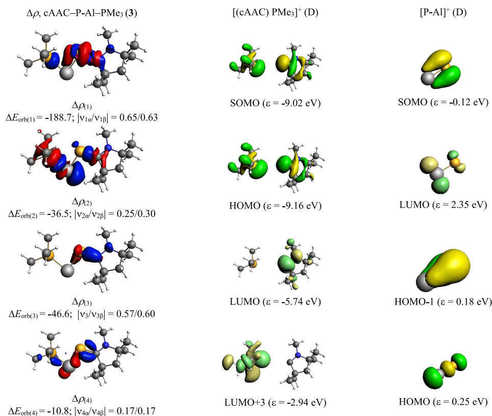
Figure 3. Shape of the deformation densities \Delta\rho_{(1)-(4)} that correspond to \Delta E_{\text{orb}(1)-(4)} and the associated MOs of \text{cAAC-PAl-PMe}_3 ( 3 ) and the fragments orbitals of [(\text{cAAC}) (\text{PMe}_3)]^+ and [\text{P-Al}] in the doublet state ( D ) at the BP86-D3(BJ)/TZ2P level. Isosurface values are 0.003 au for \Delta\rho_{(1)-(3)} and 0.001 for \Delta\rho_{(4)} . The eigenvalues |v_n| give the size of the charge migration in e. The direction of the charge flow of the deformation densities is red \rightarrow blue.
