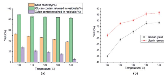
Fig. 1 Pretreatment condition: 4 g corn stover in 40 mL (80 vol% ethylene glycol) solution at 0.6 wt% H 2 SO 4 (w/w) for 60 min. (a) Effect of pretreatment temperature on solid recovery, glucan and xylan content retained in residual. (b) Effect of pretreatment temperature on enzymatic hydrolysis of cellulose and the removal of lignin.
