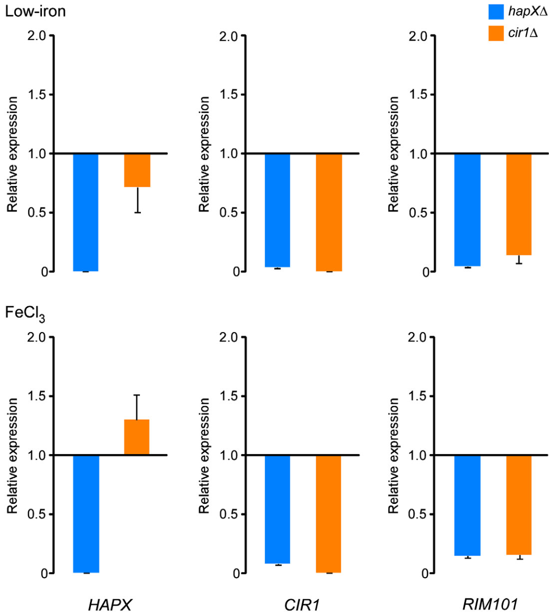
Figure 4. HapX positively regulates the levels of the CIR1 and RIM101 transcripts. Quantification of HAPX , CIR1 and RIM101 transcripts by quantitative RT-PCR in WT, hapX Δ and cir1 Δ strains under low-iron (top) and iron-replete (bottom) conditions. The data were normalized using 18S rRNA as an internal control and are presented as relative expression in comparison to the WT value set at 1. The data are from three biological and two technical replicates, and the bars represent standard deviations. doi:10.1371/journal.ppat.1001209.g004
