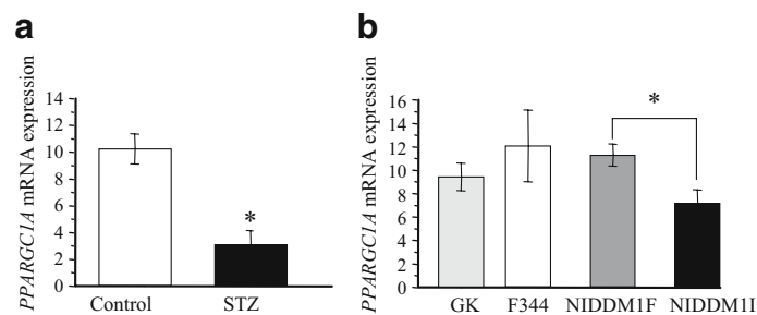
Fig. 3 PPARGC1A mRNA expression in rodent pancreatic islets. a Male Wistar rats (2–3 months old) were treated with STZ-NA ( n=5 ) or vehicles (control; n=5 ) [10, 11] and PPARGC1A mRNA expression together with the internal standard cyclophilin A was analysed in pancreatic islets isolated from STZ-NA-treated animals showing a stable hyperglycaemia (8.9–10.0 mmol glucose/l) and controls. b PPARGC1A mRNA expression together with the internal standard cyclophilin A was analysed in pancreatic islets prepared from rats at 8 weeks of age after a 6 h fast. GK rats ( n=6 ) were obtained from the Stockholm colony and bred as described [12]. Inbred, normoglycaemic
