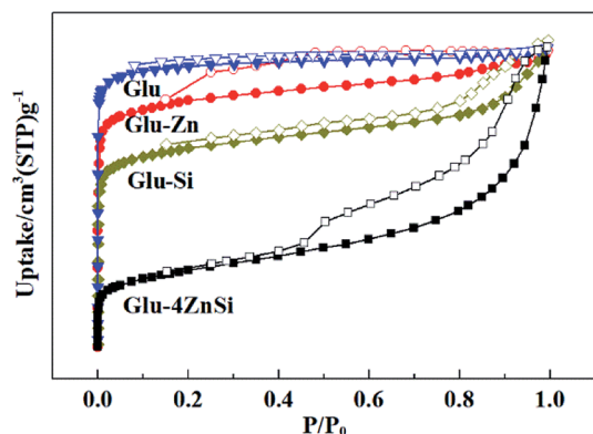
Fig. 3 Nitrogen adsorption-desorption isotherms of the carbon materials.
