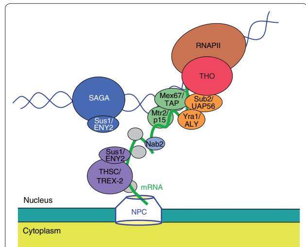
Figure 1. The THO complex functions in mRNP biogenesis at the interface between transcription and export of mRNA from the nucleus. Proteins are shown with their yeast name followed by the name of the human homolog, where the two differ, for Nab2, Mtr2/p15, Sub2/UAP56, Mex67/TAP, Yra1/ALY, or with the yeast name followed by the Drosophila name for Sus1/ENY2. Protein complexes are shown in capital letters: THO, THSC (also called TREX-2) and SAGA. Proteins that interact with each other or between which a physical connection has been reported are in the same color. Sus1 can act as a subunit of both THSC and SAGA complexes. Unlabeled proteins in gray represent other factors important for mRNP biogenesis and export. NPC, nuclear pore complex; RNAPII, RNA polymerase II.
