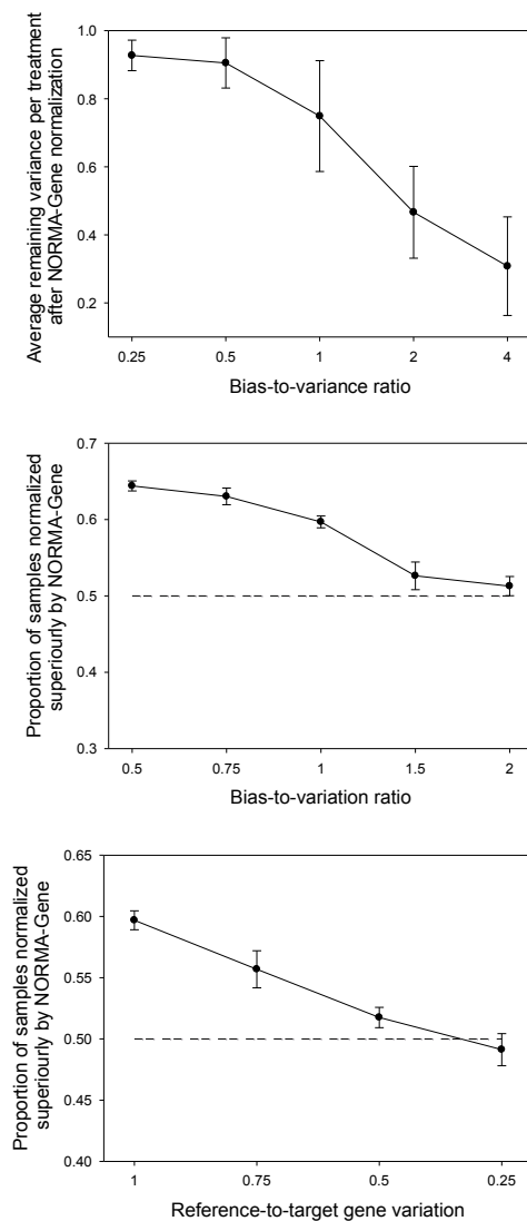
Figure 2 The figure shows the results of analysis of artificial data-sets. Throughout means \pm SEM of the 40 re-samplings are given. Top panel: This panel shows the variance reduction by normalization and how this depends on the bias-to-variation ratio. Increasing the bias-to-variation ratio in the artificial data leads to more variance being removed from the data-set by NORMA-Gene. Middle and bottom panels: These panels show the effectiveness of NORMA-Gene versus reference gene normalization and the dependence of different parameters. For each of the re-samplings (see methods for detailed information on the construction of the data-sets) the proportion of NORMA-Gene normalized data points that were closer to the true mean was calculated and is shown on the y-axis (0.5 represent equal performance of NORMA-Gene and reference gene normalization). Middle panel: Here the x-axis represents the ratio between bias (between replicate variation) and variation (between genes within replicate variation). As bias among replicates increase the performance of NORMA-Gene decreases. No qualitative difference was observed in the performance of NORMA-Gene between re-sampling from eight or four genes. Bottom panel: The x-axis represents the ratio of reference gene-to-target gene variation (here 1 represent equal variation and 0.25 represent four-fold decreased variation in the reference factor).
