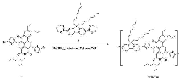
Scheme 1 Synthetic route of PF8NT2/6.
