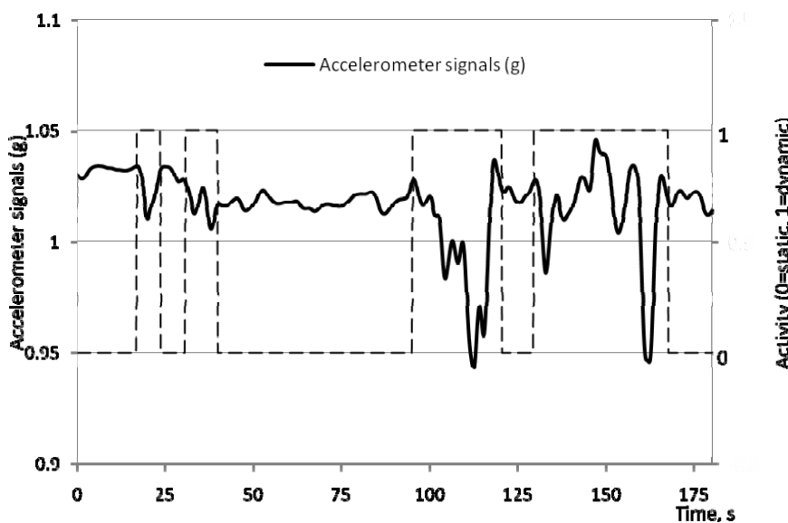
Figure 3 Plot of the resultant accelerometer signals against time. The period when the signals exceed the threshold (shown as dotted line with a value of 1) was defined as dynamic activities.
