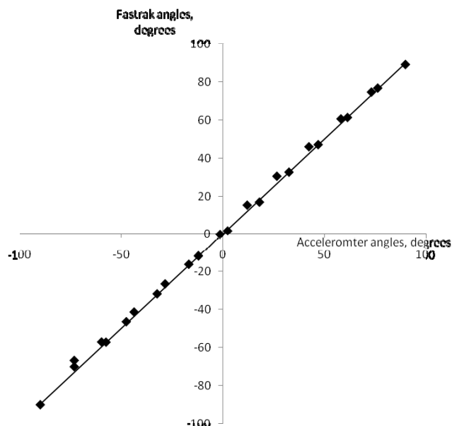
Figure 2 Plot of fastrak angles against angles derived from the accelerometers with the best straight line fit.
