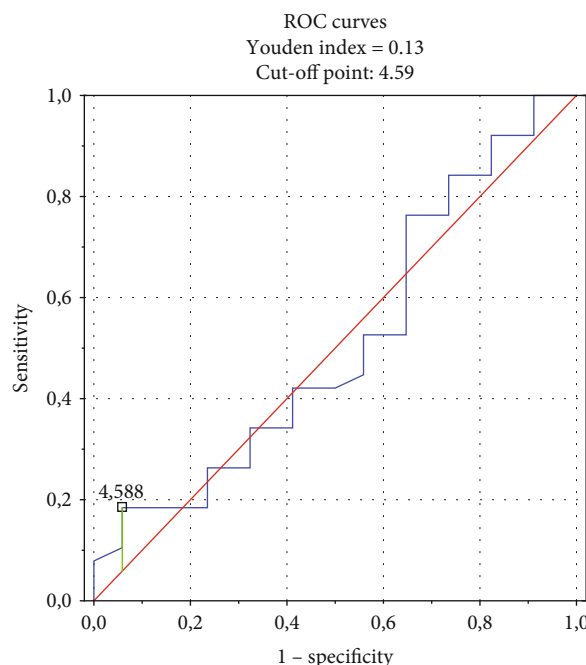
FIGURE 1: The ROC curves present sensitivity and specificity of NLR in predicting the spatial QRS-T angle.
