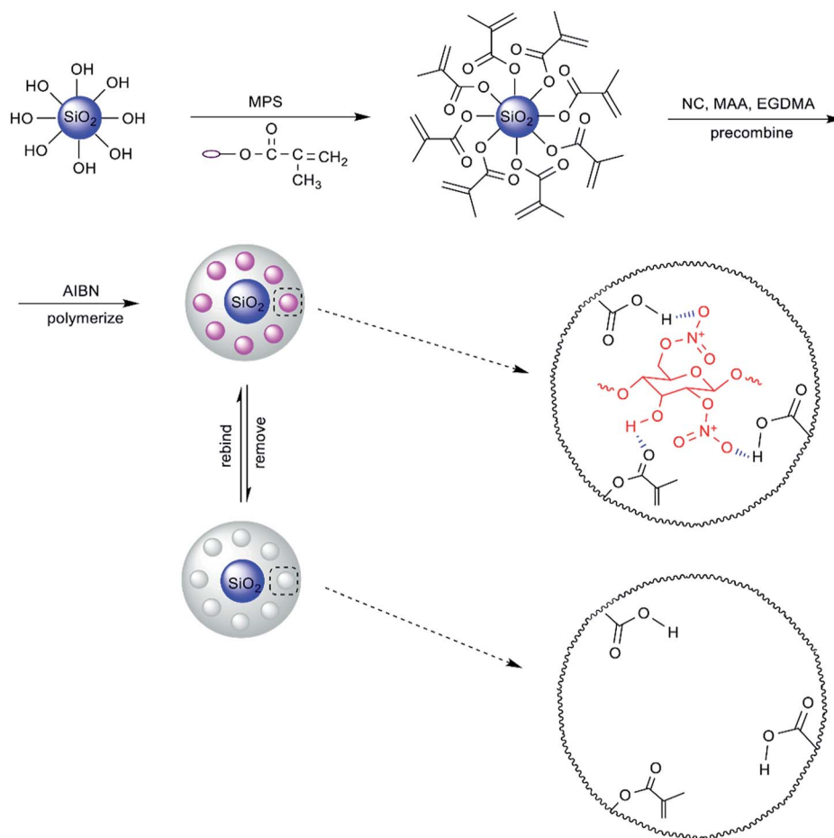
Fig. 1 Schematic diagram of the imprinting process of nitrocellulose on the surface of SiO 2 .
