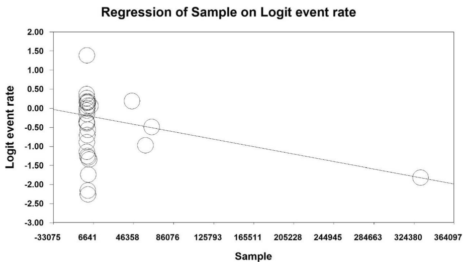
Fig. 5 Meta-regression diagram of the overall prevalence of urinary incontinence in older adults' women worldwide by sample size
