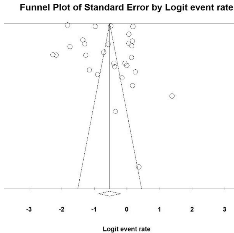
Fig. 2 Funnel Plot Results of urinary incontinence in older adults' women worldwide
