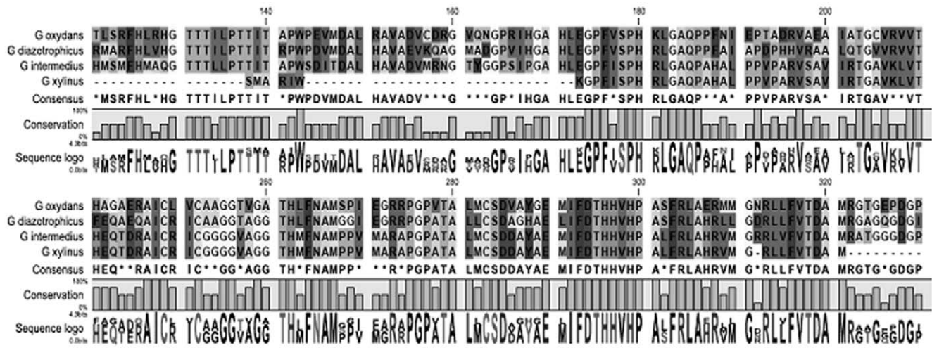
Figure 1. Multiple-amino-acid alignment of nagA proteins from G. xylinus and from other bacteria. Putative amino acid sequence of nagA homolog of G. xylinus , nagA of G. intermedius (Genbank access. no. BAI39462), nagA of G. diazotrophicus Pal 5 (YP_001602823), nagA of G. oxydans 621 H (YP_001602823).
