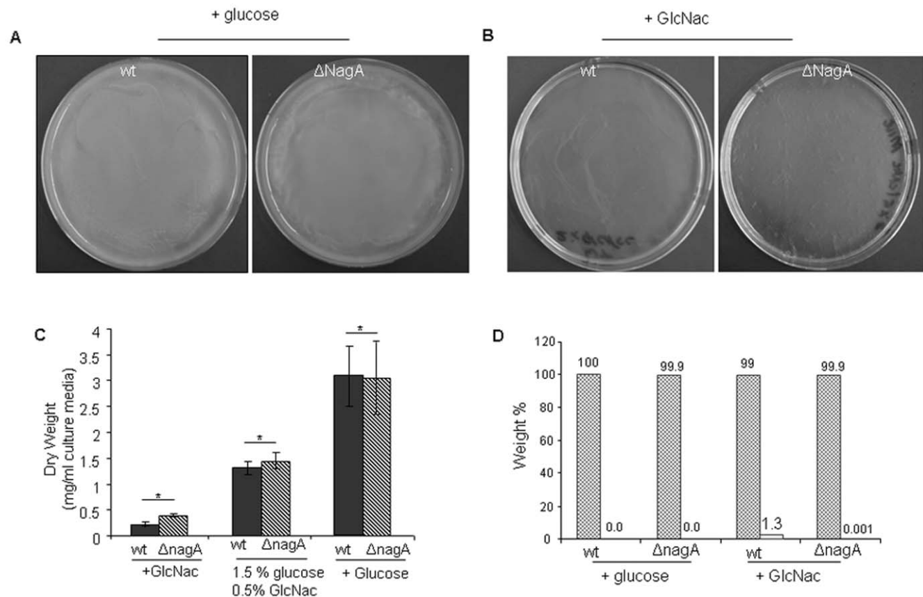
Figure 5. Cellulose production and pellicle morphology. (a) Morphological appearance of cellulose pellicles produce after one week by wild type and \Delta NagA G. xylinus in the presence of either (A) glucose; or (B) GlcNAc as carbon source. (C) Cellulose production efficiency of wild type and \Delta NagA G. xylinus supplemented with either glucose, GlcNAc or both as carbon source. Error bar represent s.d. of three replicates (* p < 0.001 ); (D) Quantitative LC-MS/MS for quantification and relative weight percent (wt%) of glucose and GlcNAc in acid hydrolyzed cellulose extruded from wild type or \Delta NagA fed with either glucose or GlcNAc. Error bar represent s.d. of three replicates (* p < 0.001 ). (E) Linear regression curve for known glucose; and (F) for known GlcNAc to quantify glucose and GlcNAc in acid hydrolyzed cellulose samples by LC-MS/MS. doi:10.1371/journal.pone.0018099.g005
