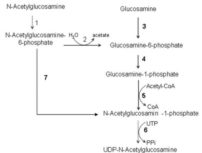
Figure 6. UDP-GlcNAc biosynthetic pathway in bacteria (including G. xylinus ) and eukaryotes. Reactions with open arrows occur in bacteria and reactions with filled arrow occur in eukaryotes while dotted arrow reactions are common in both bacteria and animals. Enzymes involved are as follows; 1: N-acetylglucosamine kinase; 2: N-acetylglucosamine-6-phosphate deacetylase; 3: Glucosamine kinase; 4: Phosphoglucosamine mutase; 5: Glucosamine-6-phosphate N-acetyltransferase; 6: UDP-N-acetylglucosamine pyrophosphorylase; 7: Phosphoacetylglucosamine mutase.
