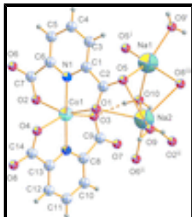
Fig. 1. The asymmetric unit of the title compound. Displacement ellipsoids are shown at the 50% probability level. Hydrogen bonds are indicated by dashed lines. [Symmetry codes: (i) 1/2+x, 1/2-y, z ; (ii) -x, -y, 1/2+z ; (iii) -1/2-x, 1/2+y, 1/2+z .]
