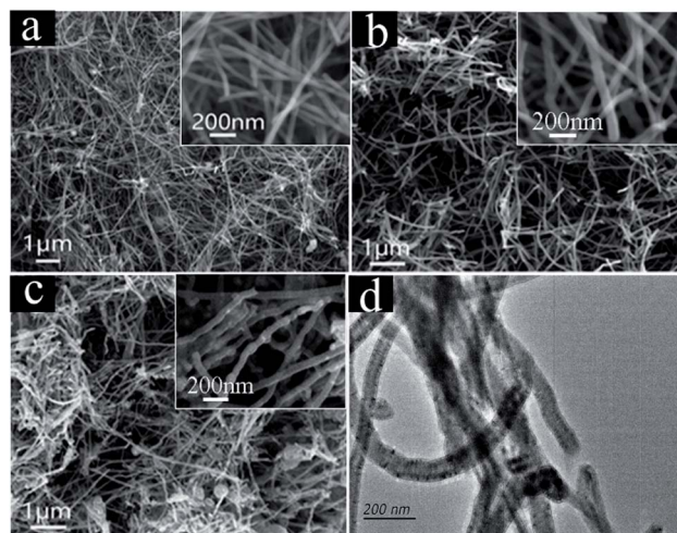
Fig. 4 SEM images of carbon products obtained in 750 °C Li_2CO_3 electrolyte: (a) 50 mA\text{ cm}^{-2} , (b) 100 mA\text{ cm}^{-2} , (c) 300 mA\text{ cm}^{-2} , (d) TEM of CNTs prepared at 100 mA\text{ cm}^{-2} .
