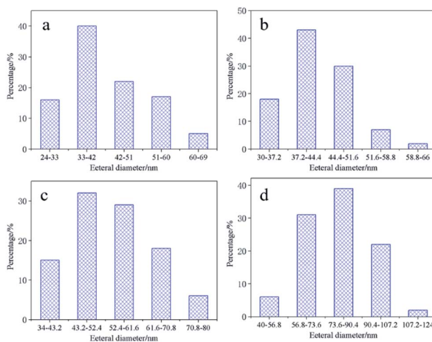
Fig. 5 The outer diameter distribution of CNTs obtained under different current densities in 750 °C Li_2CO_3 electrolyte (a) 50 mA\text{ cm}^{-2} , (b) 100 mA\text{ cm}^{-2} , (c) 200 mA\text{ cm}^{-2} , (d) 300 mA\text{ cm}^{-2} .
